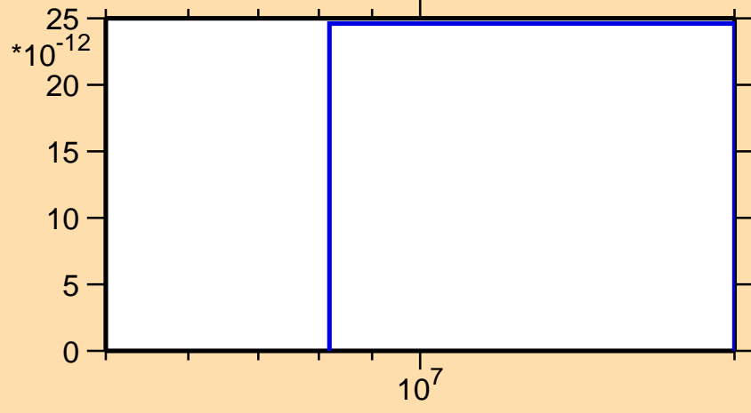
\sigma vs. E for ^{200}\text{Hg}(n,\text{nd})
