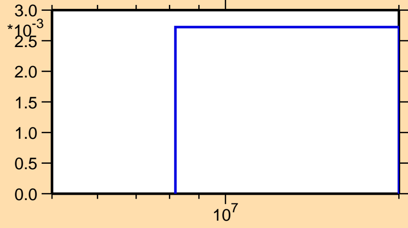
\sigma vs. E for ^{200}\text{Hg}(n,3n)
