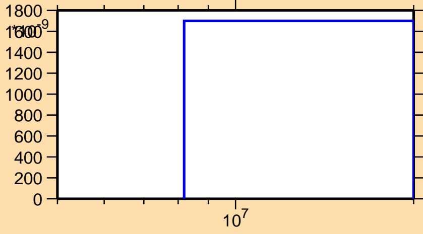
\sigma vs. E for ^{200}\text{Hg}(n,t)
