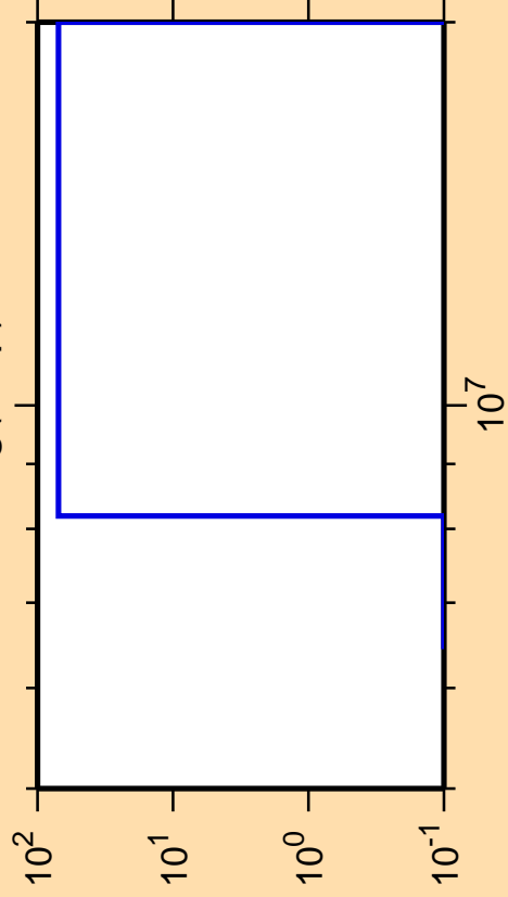
\Delta\sigma/\sigma vs. E for ^{200}\text{Hg}(n,np)
