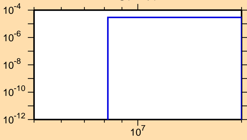
\sigma vs. E for ^{200}\text{Hg}(n,np)
