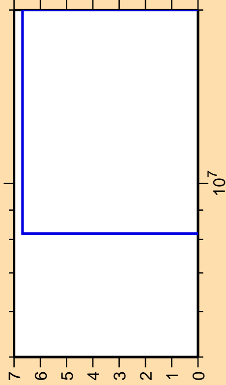
\Delta\sigma/\sigma vs. E for ^{200}\text{Hg}(n,nt)
