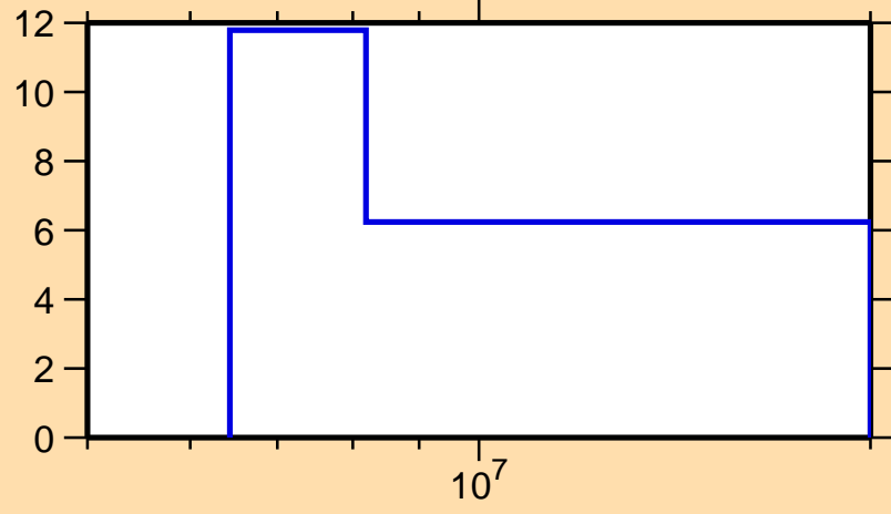
\Delta\sigma/\sigma vs. E for ^{200}\text{Hg}(n,\text{el.})
