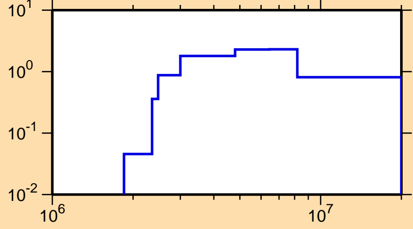
\sigma vs. E for ^{200}\text{Hg}(n,n\text{cont.})
