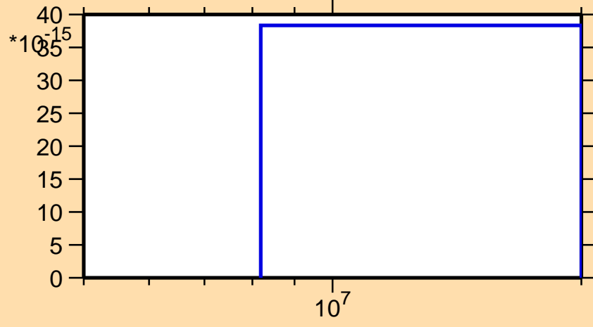
\sigma vs. E for ^{200}\text{Hg}(n,\text{He}3)
