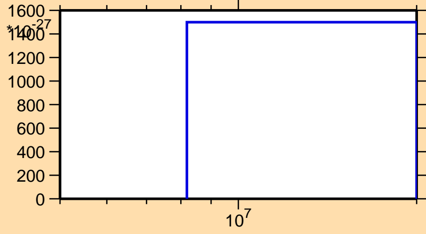
\sigma vs. E for ^{200}\text{Hg} (mt 11)
