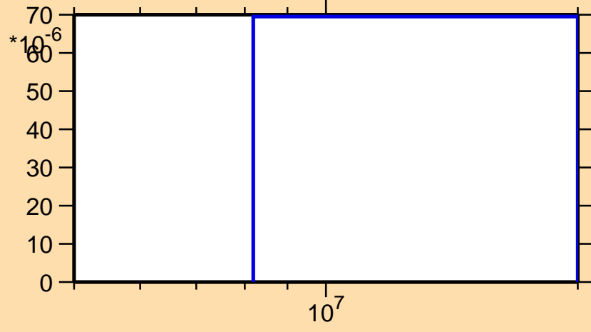
\sigma vs. E for ^{200}\text{Hg}(n,d)
