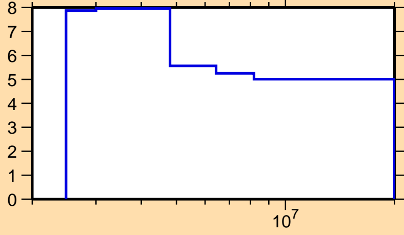
\Delta\sigma/\sigma vs. E for ^{200}\text{Hg}(n,\text{nonel.})
