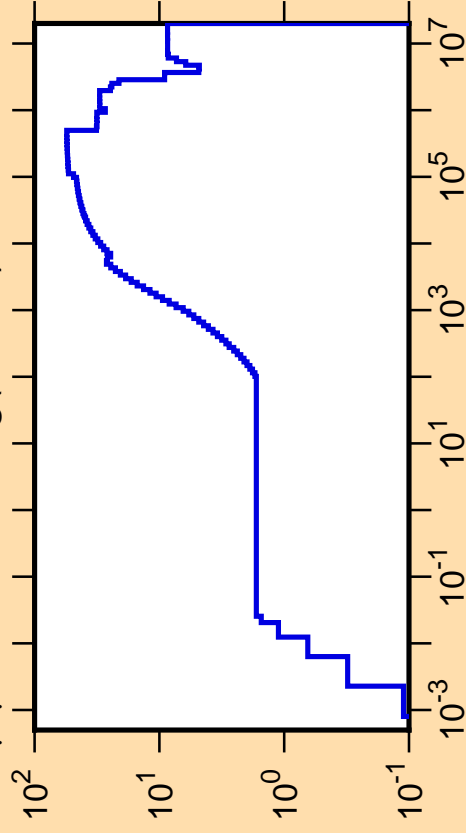
\Delta\mu/\mu vs. E for ^{201}\text{Hg}(\text{mt251})
