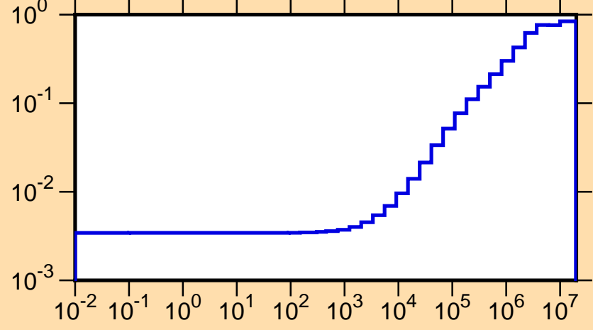
\mu vs. E for ^{201}\text{Hg}(\text{mt251})
