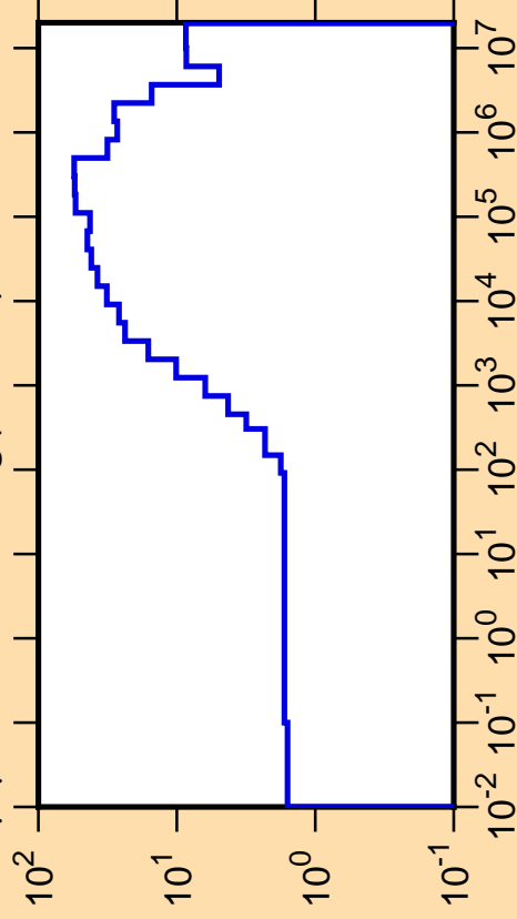
\Delta\mu/\mu vs. E for ^{201}\text{Hg}(\text{mt251})
