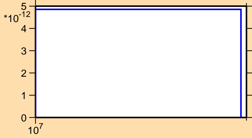
\sigma vs. E for ^{201}\text{Hg}(n,\text{nt})
