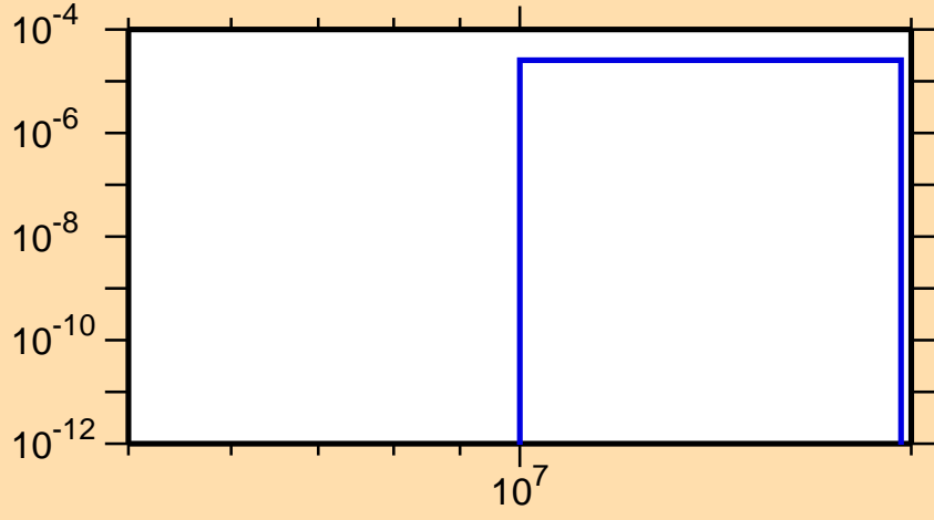
\sigma vs. E for ^{201}\text{Hg}(n,np)
