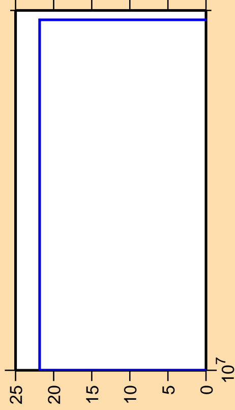
\Delta\sigma/\sigma vs. E for ^{201}\text{Hg}(n,\text{nt})
