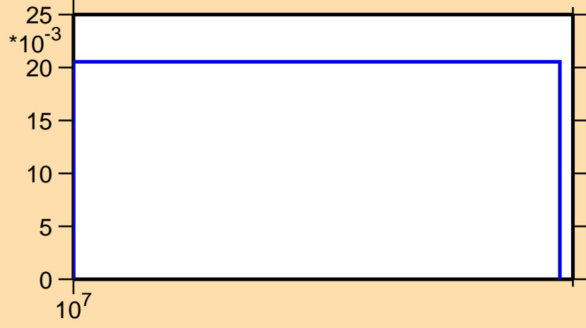
\sigma vs. E for ^{201}\text{Hg}(n,3n)
