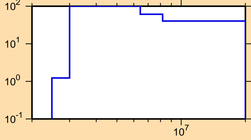
\Delta\sigma/\sigma vs. E for ^{201}\text{Hg}(n,p)
