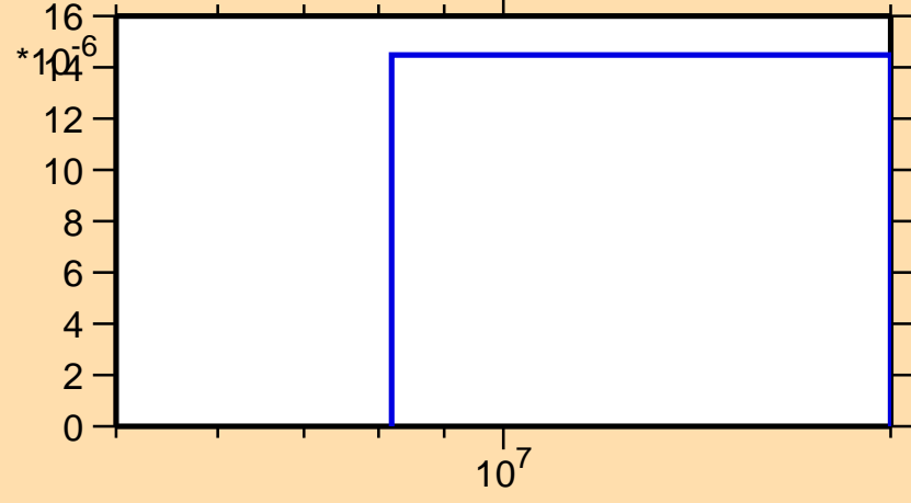
\sigma vs. E for ^{201}\text{Hg}(n,t)
