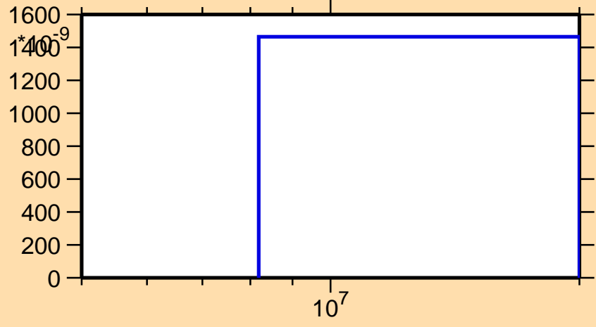
\sigma vs. E for ^{201}\text{Hg}(n,\alpha)
