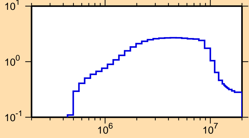
\sigma vs. E for ^{202}\text{Hg}(n,\text{inel.})
