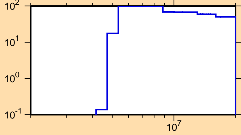
\Delta\sigma/\sigma vs. E for ^{202}\text{Hg}(n,p)
