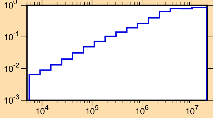
\mu vs. E for ^{202}\text{Hg}(\text{mt251})
