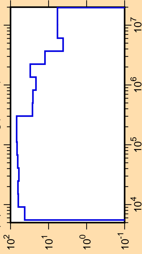
\Delta\mu/\mu vs. E for ^{202}\text{Hg}(\text{mt251})
