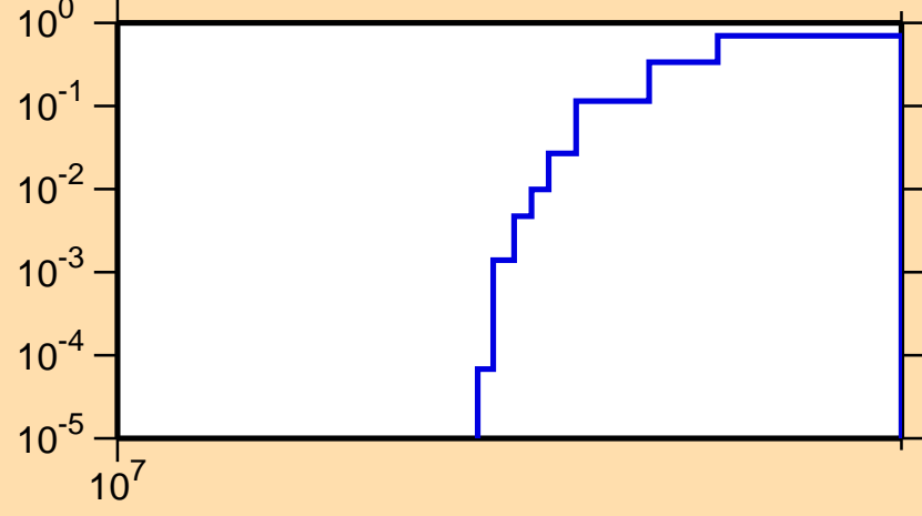
\sigma vs. E for ^{203}\text{Hg}(n,3n)
