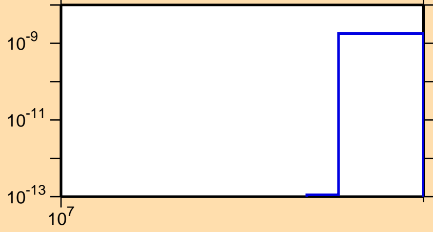
\sigma vs. E for ^{203}\text{Hg}(n,2np)
