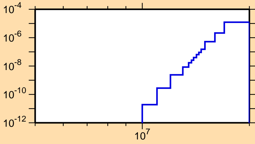
\sigma vs. E for ^{203}\text{Hg}(n,n\alpha)
