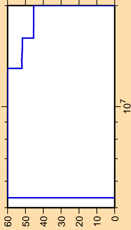
\Delta\sigma/\sigma vs. E for ^{203}\text{Hg}(n,p)
