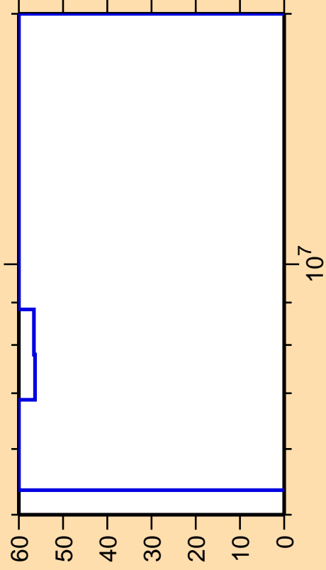
\Delta\sigma/\sigma vs. E for ^{203}\text{Hg}(n,\gamma)
