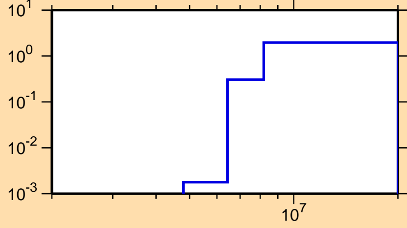
\sigma vs. E for ^{203}\text{Hg}(n,2n)
