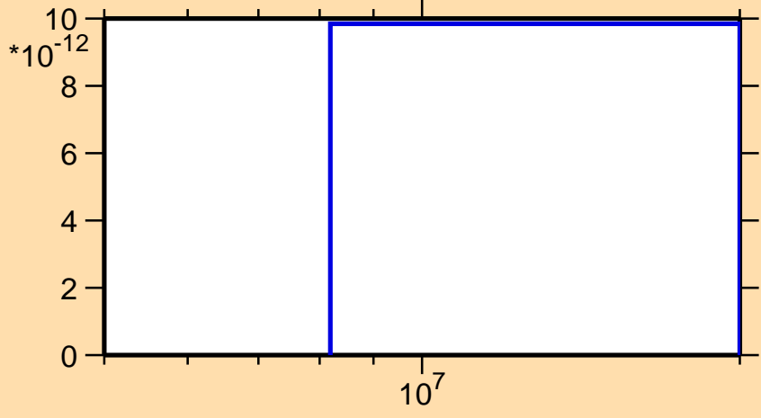
\sigma vs. E for ^{203}\text{Hg}(n,\text{nt})
