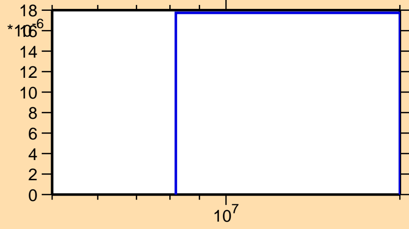
\sigma vs. E for ^{203}\text{Hg}(n,np)
