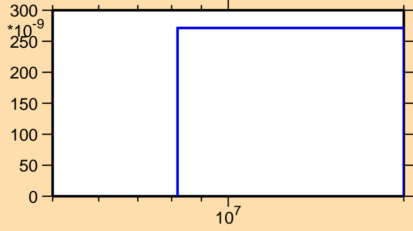
\sigma vs. E for ^{203}\text{Hg}(n,\alpha)
