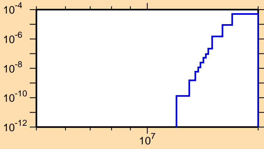
\sigma vs. E for ^{204}\text{Hg}(n,t)
