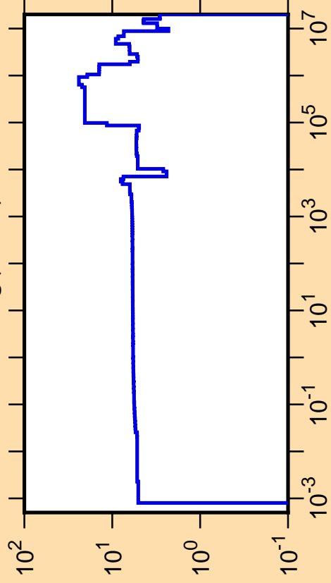
\Delta\sigma/\sigma vs. E for ^{204}\text{Hg}(n,\text{tot.})
