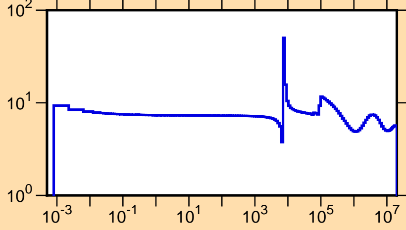
\sigma vs. E for ^{204}\text{Hg}(n,\text{tot.})
