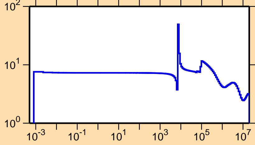
\sigma vs. E for ^{204}\text{Hg}(n,\text{el.})
