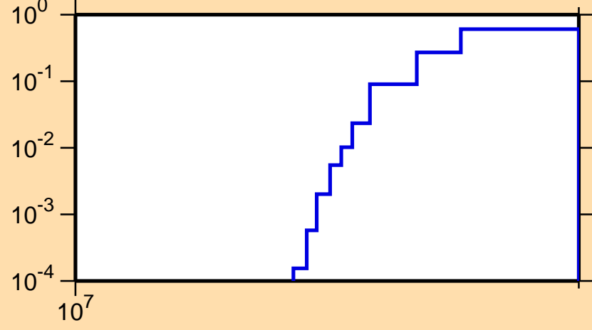
\sigma vs. E for ^{204}\text{Hg}(n,3n)
