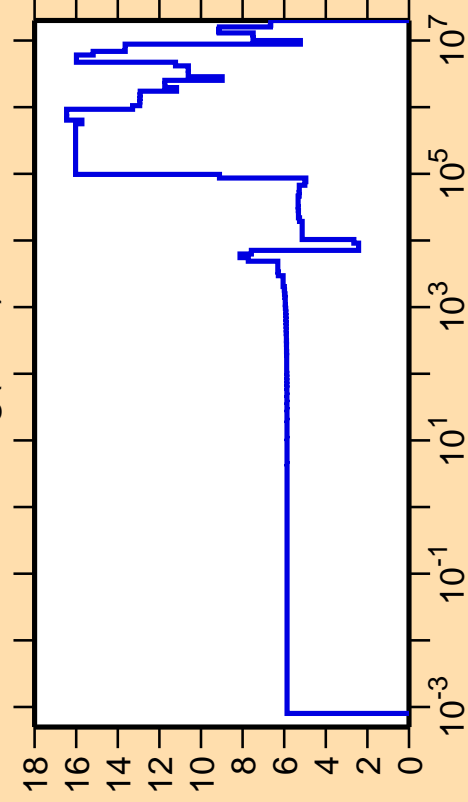
\Delta\sigma/\sigma vs. E for ^{204}\text{Hg}(n,\text{el.})
