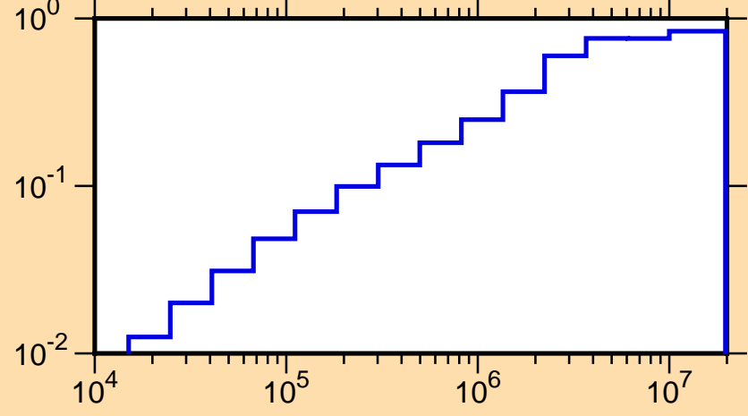
\mu vs. E for ^{204}\text{Hg}(\text{mt251})
