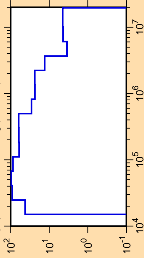
\Delta\mu/\mu vs. E for ^{204}\text{Hg}(\text{mt251})
