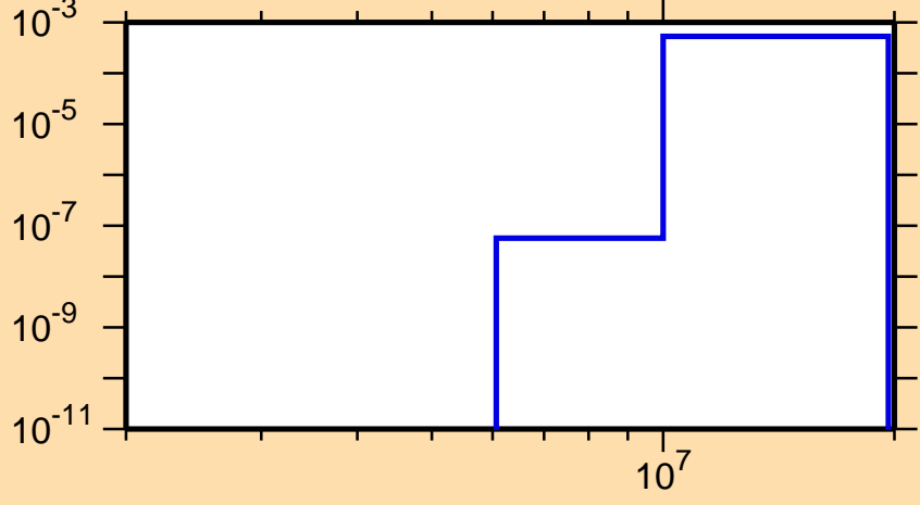
\sigma vs. E for ^{204}\text{Hg}(n,p)
