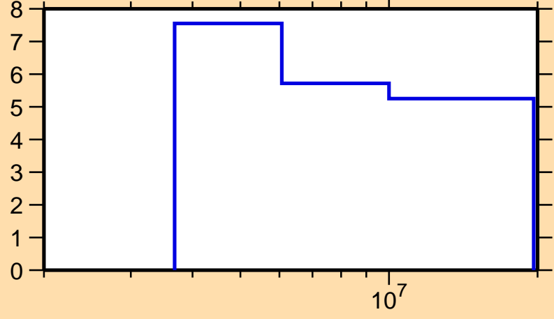
\Delta\sigma/\sigma vs. E for ^{204}\text{Hg}(n,\text{nonel.})
