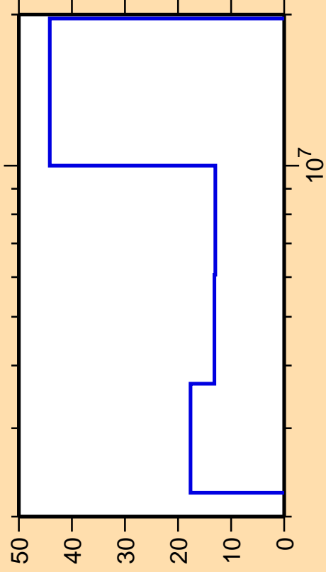
\Delta\sigma/\sigma vs. E for ^{204}\text{Hg}(n,\text{ncont.})
