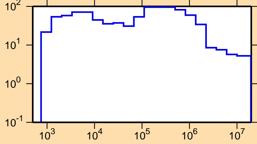
\Delta\sigma/\sigma vs. E for ^{204}\text{Hg}(n,\text{nonel.})
