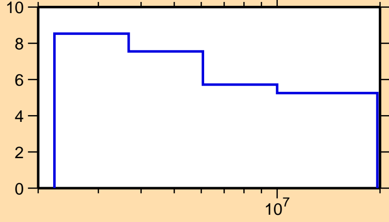
\Delta\sigma/\sigma vs. E for ^{204}\text{Hg}(n,n\text{onel.})
