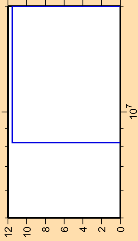
\Delta\sigma/\sigma vs. E for ^{204}\text{Hg}(n,\text{nt})
