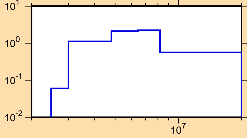
\sigma vs. E for ^{204}\text{Hg}(n,n\text{cont.})
