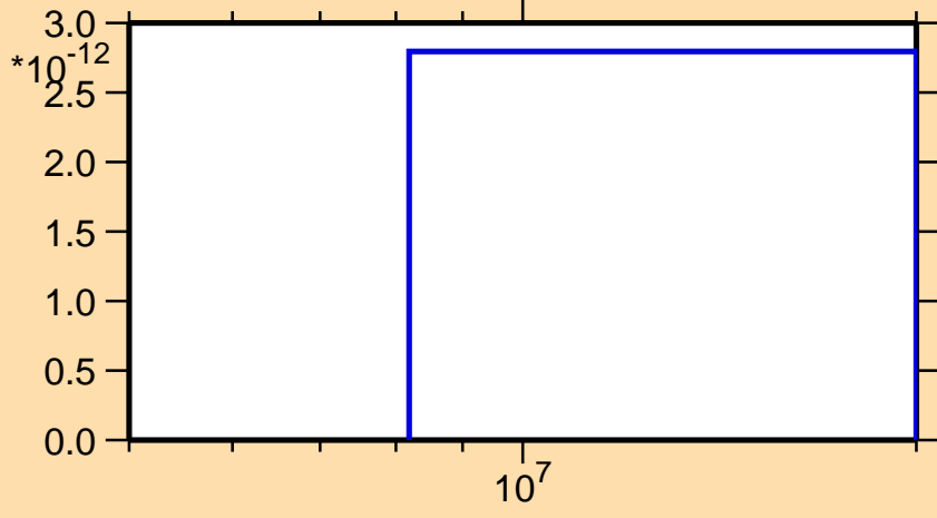
\sigma vs. E for ^{204}\text{Hg}(n,\text{nt})
