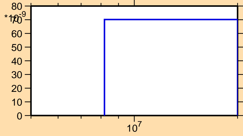
\sigma vs. E for ^{204}\text{Hg}(n,\alpha)
