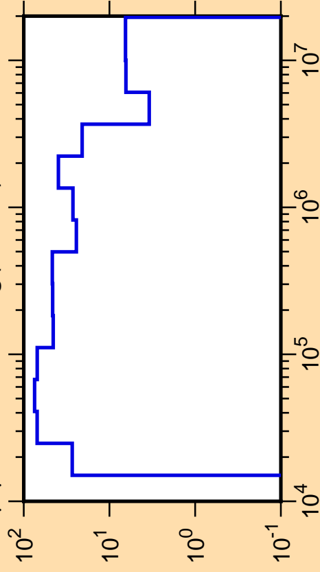
\Delta\mu/\mu vs. E for ^{205}\text{Hg}(\text{mt251})
