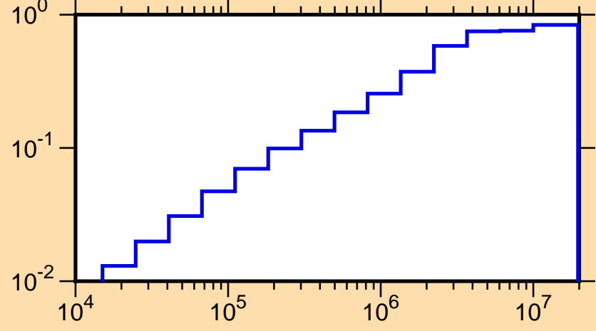
\mu vs. E for ^{205}\text{Hg}(\text{mt251})
