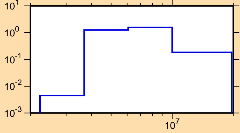
\sigma vs. E for ^{205}\text{Hg}(n,n\text{cont.})
