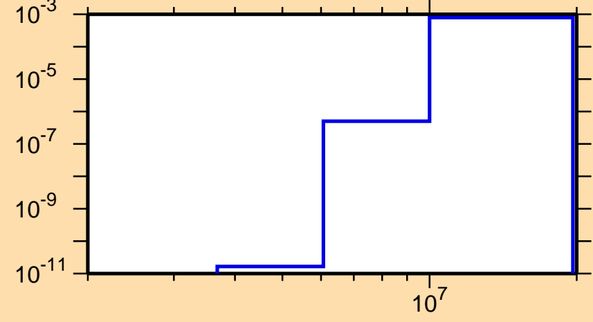
\sigma vs. E for ^{205}\text{Hg}(n,p)
