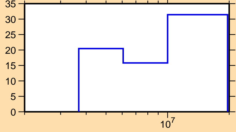
\Delta\sigma/\sigma vs. E for ^{205}\text{Hg}(n,n\text{cont.})
