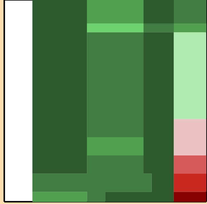
\Delta\sigma/\sigma vs. E for ^{206}\text{Hg}(n,p)
