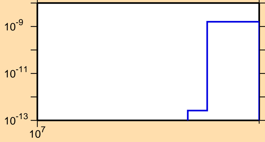
\sigma vs. E for ^{206}\text{Hg}(n,nt)
