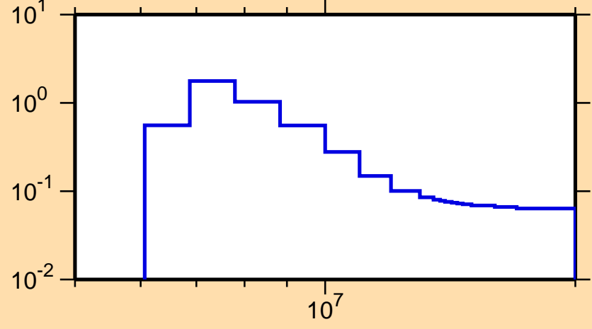
\sigma vs. E for ^{206}\text{Hg}(n,n\text{cont.})
