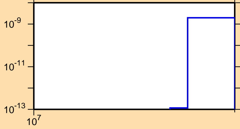
\sigma vs. E for ^{206}\text{Hg}(n,\text{nd})
