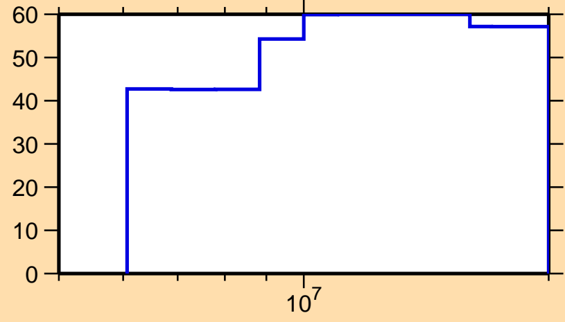
\Delta\sigma/\sigma vs. E for ^{206}\text{Hg}(n,ncont.)
