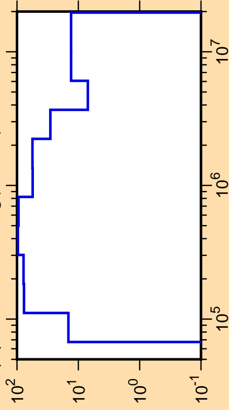
\Delta\mu/\mu vs. E for ^{206}\text{Hg}(\text{mt251})
