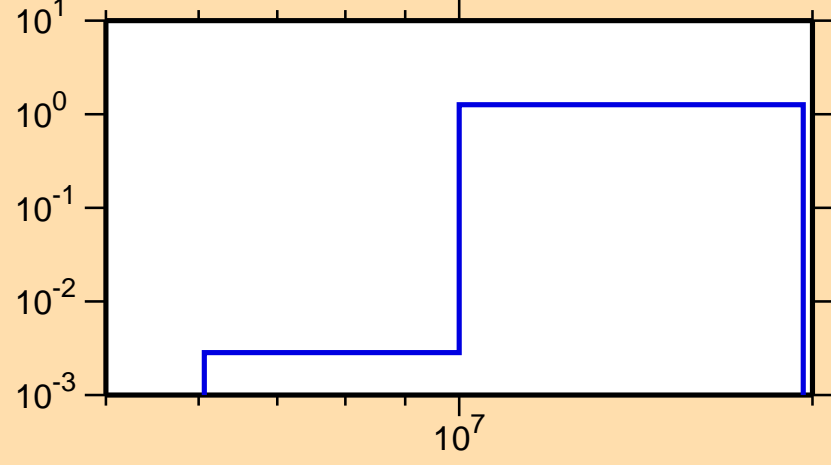
\sigma vs. E for ^{208}\text{Hg}(n,3n)
