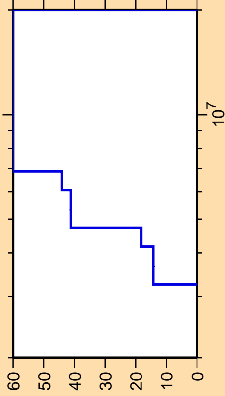
\Delta\sigma/\sigma vs. E for ^{209}\text{Hg}(n,n\text{cont.})
