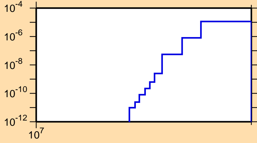
\sigma vs. E for ^{209}\text{Hg}(n,\text{nt})
