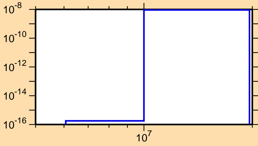
\sigma vs. E for ^{209}\text{Hg}(n,2n\alpha)
