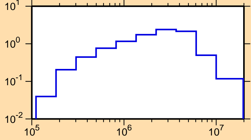
\sigma vs. E for ^{209}\text{Hg}(n,\text{inel.})
