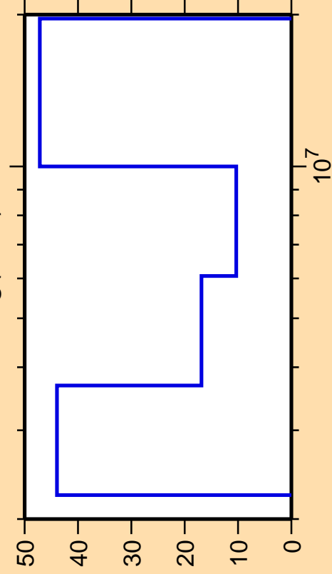
\Delta\sigma/\sigma vs. E for ^{209}\text{Hg}(n,2n)
