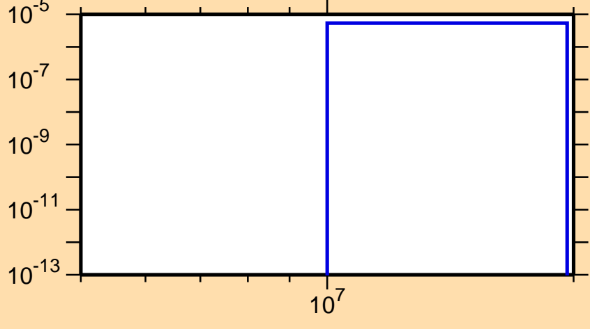
\sigma vs. E for ^{209}\text{Hg}(n,d)
