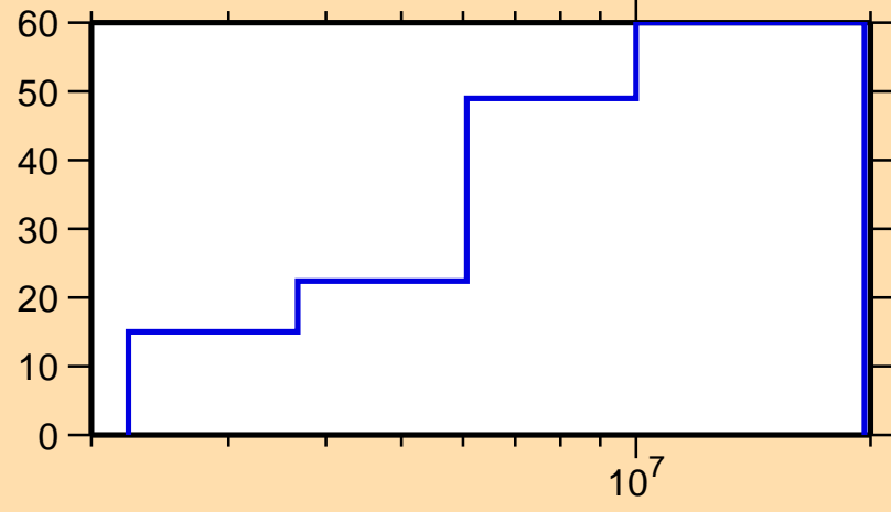
\Delta\sigma/\sigma vs. E for ^{209}\text{Hg}(n,n\text{cont.})
