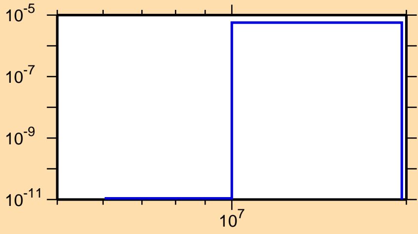
\sigma vs. E for ^{209}\text{Hg}(n,\alpha)
