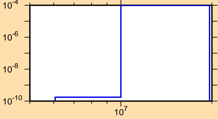
\sigma vs. E for ^{209}\text{Hg}(n,p)
