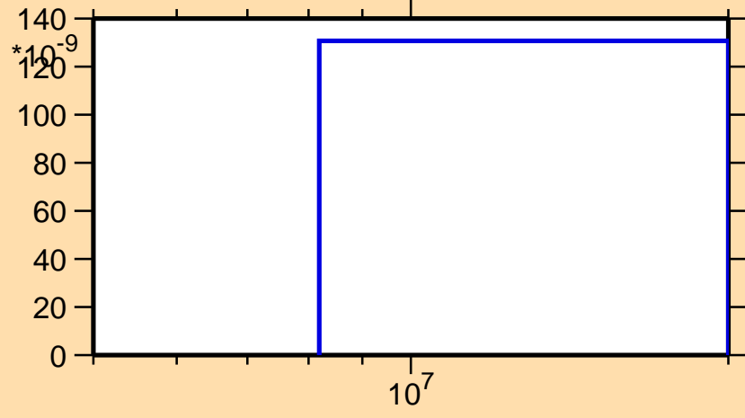
\sigma vs. E for ^{209}\text{Hg}(n,\text{nt})
