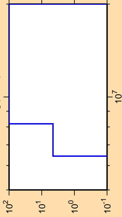
\Delta\sigma/\sigma vs. E for ^{209}\text{Hg}(n,n\alpha)
