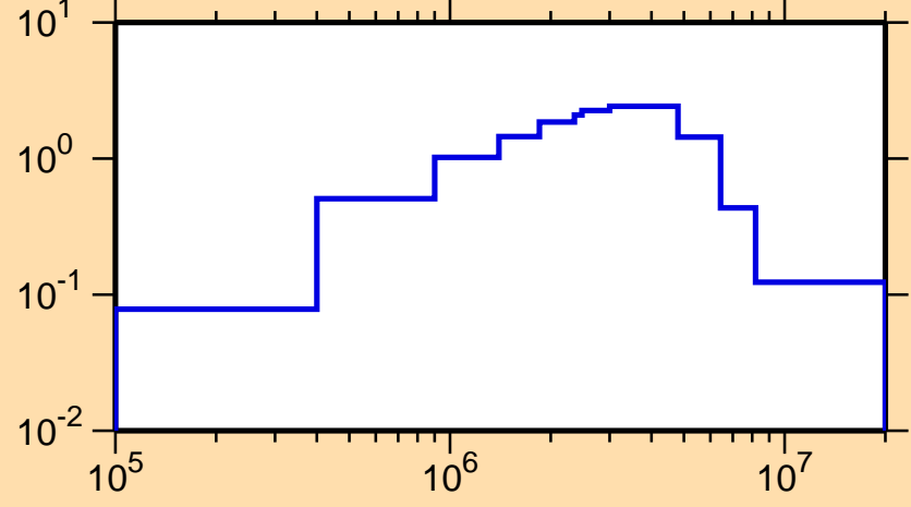
\sigma vs. E for ^{209}\text{Hg}(n,n\text{cont.})
