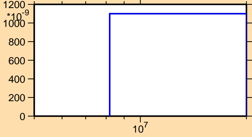
\sigma vs. E for ^{209}\text{Hg}(n,np)
