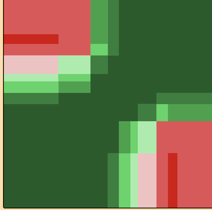
\sigma vs. E for ^{209}\text{Hg}(n,\text{inel.})
