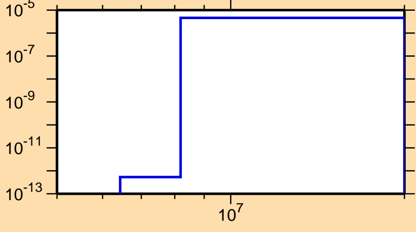
\sigma vs. E for ^{209}\text{Hg}(n,n\alpha)
