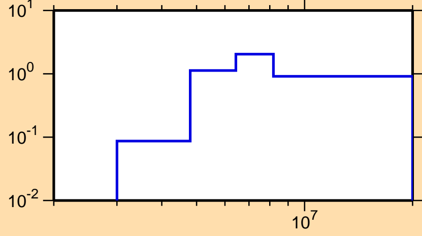
\sigma vs. E for ^{209}\text{Hg}(n,2n)
