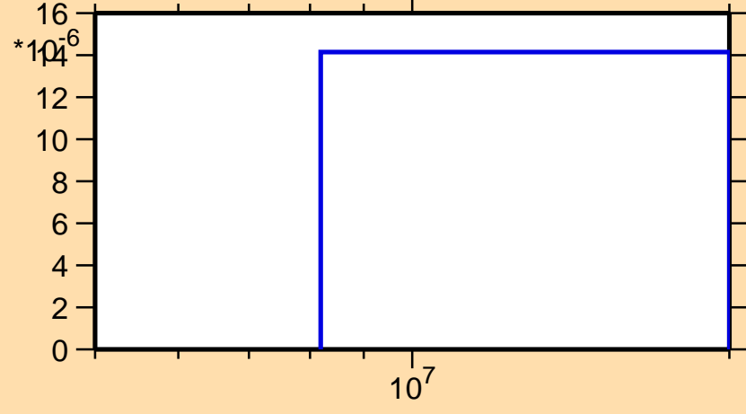
\sigma vs. E for ^{209}\text{Hg}(n,t)
