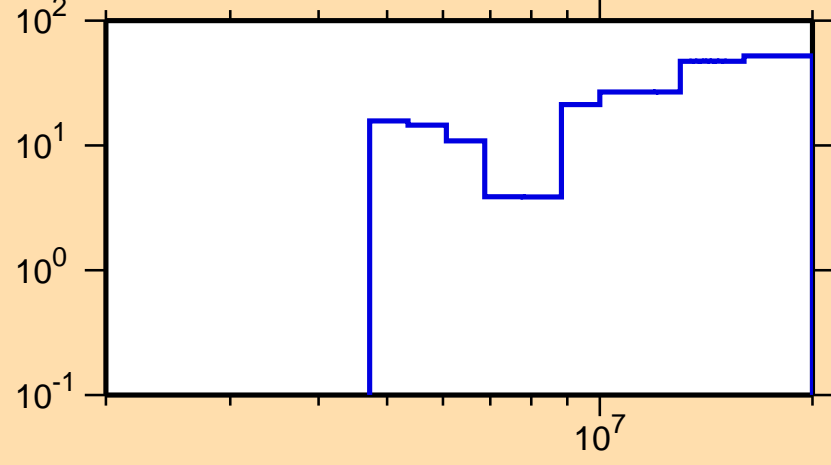
\Delta\sigma/\sigma vs. E for ^{210}\text{Hg}(n,2n)
