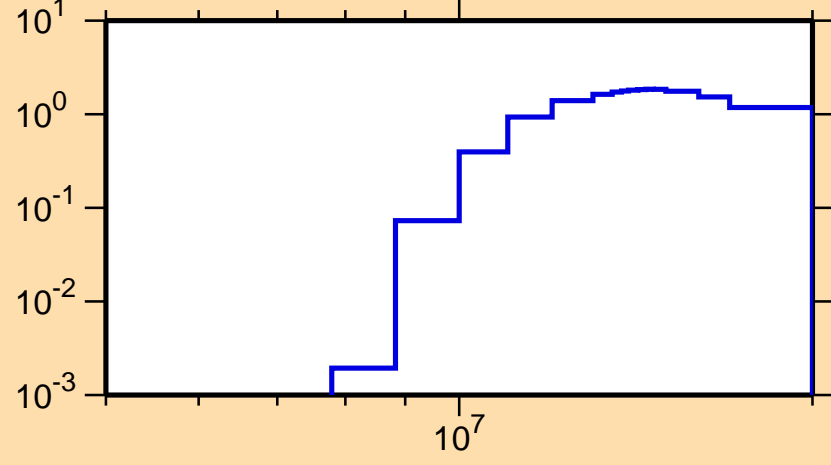
\sigma vs. E for ^{210}\text{Hg}(n,3n)
