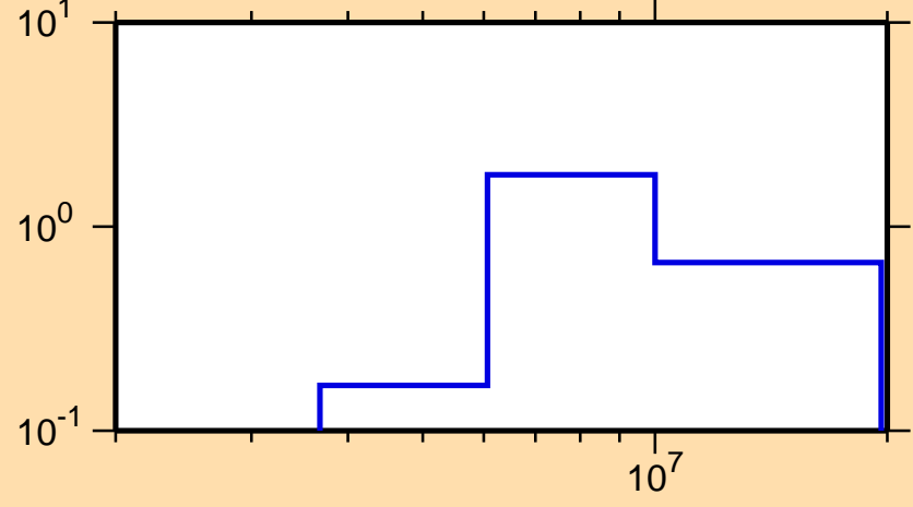
\sigma vs. E for ^{210}\text{Hg}(n,2n)
