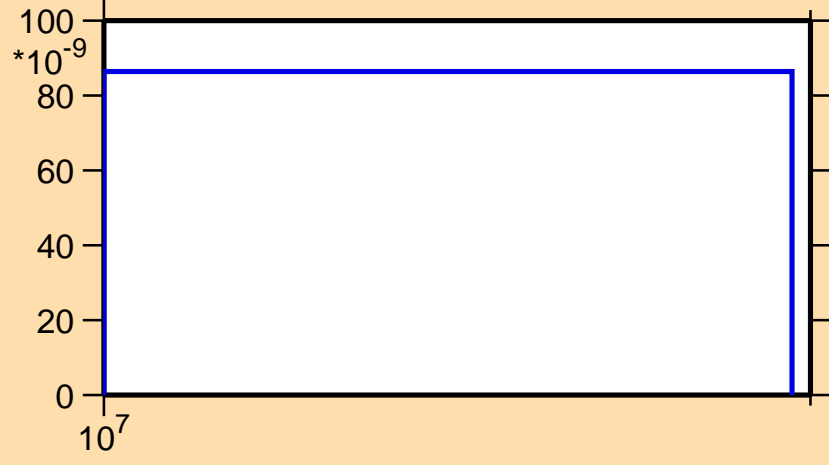
\sigma vs. E for ^{210}\text{Hg}(n,nt)
