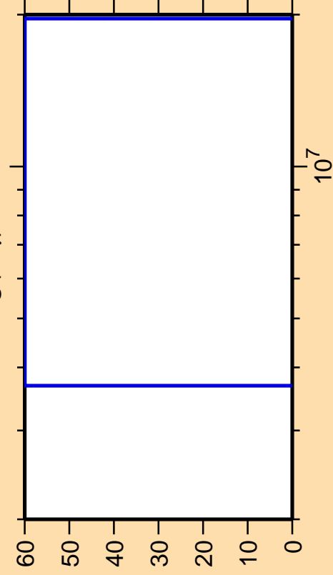
\Delta\sigma/\sigma vs. E for ^{210}\text{Hg}(n,\gamma)
