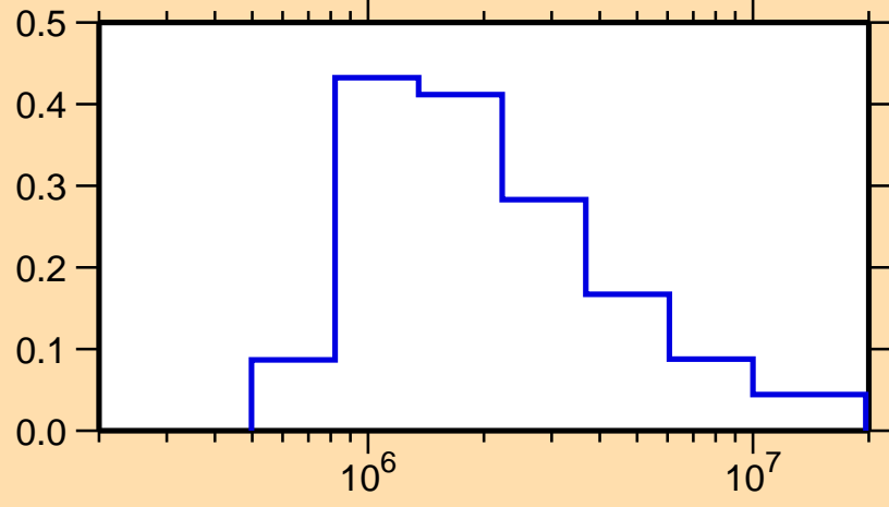
\sigma vs. E for ^{210}\text{Hg}(n,n_1)
