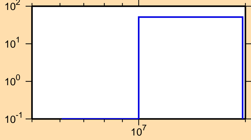
\Delta\sigma/\sigma vs. E for ^{210}\text{Hg}(n,p)
