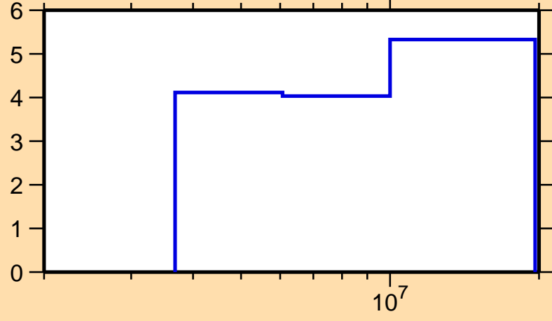
\Delta\sigma/\sigma vs. E for ^{210}\text{Hg}(n,\text{nonel.})
