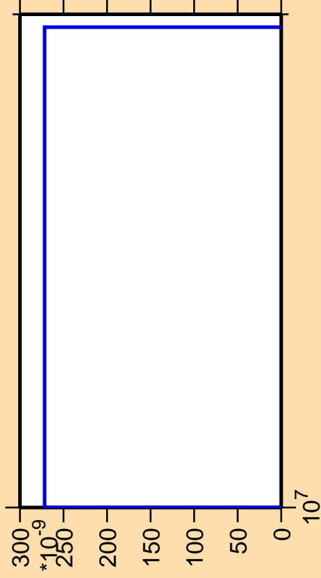
\Delta\sigma/\sigma vs. E for ^{210}\text{Hg} (mt 42)
