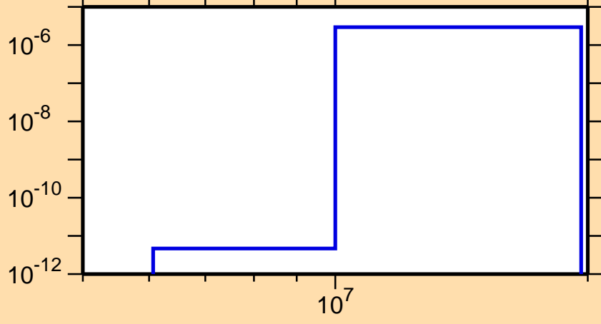
\sigma vs. E for ^{210}\text{Hg}(n,n\alpha)
