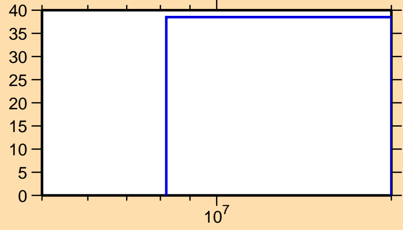
\Delta\sigma/\sigma vs. E for ^{210}\text{Hg}(n,ncont.)
