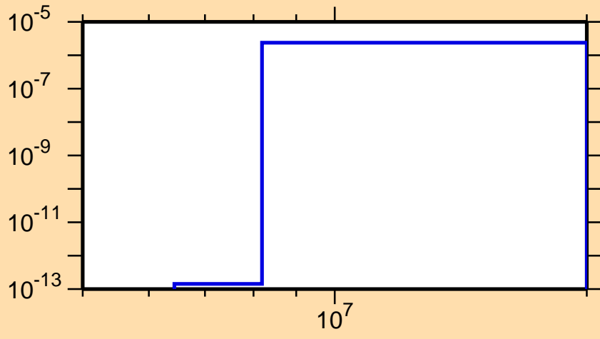
\sigma vs. E for ^{210}\text{Hg}(n,n\alpha)
