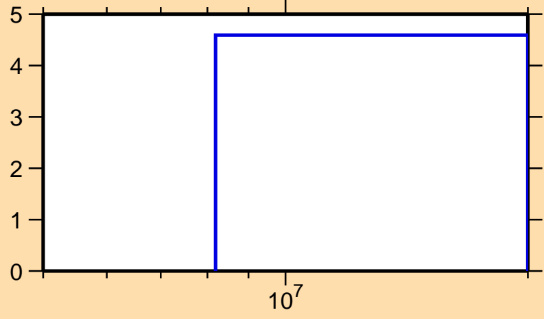
\Delta\sigma/\sigma vs. E for ^{210}\text{Hg}(n,el.)
