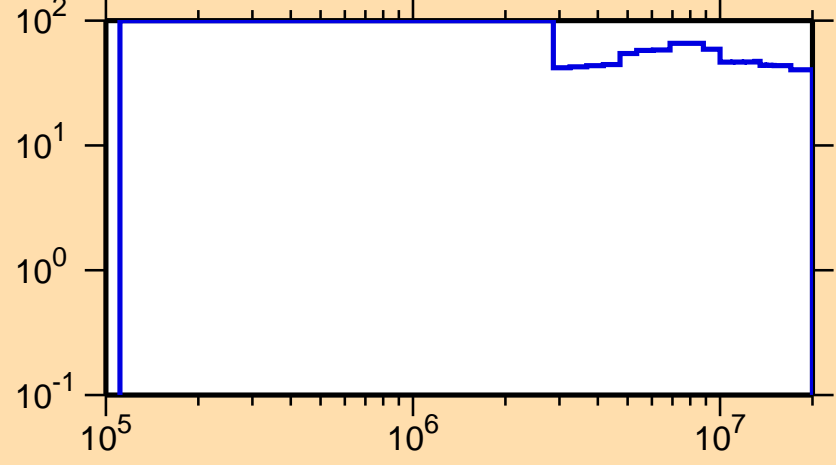
\Delta\sigma/\sigma vs. E for ^{211}\text{Hg}(n,n_1)
