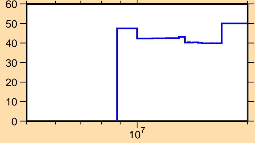
\Delta\sigma/\sigma vs. E for ^{211}\text{Hg}(n,ncont.)
