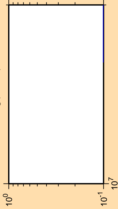
\Delta\sigma/\sigma vs. E for ^{211}\text{Hg} (mt 11)
