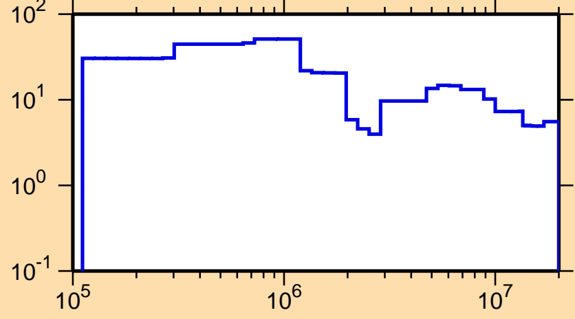
\Delta\sigma/\sigma vs. E for ^{211}\text{Hg}(n,\text{tot.})
