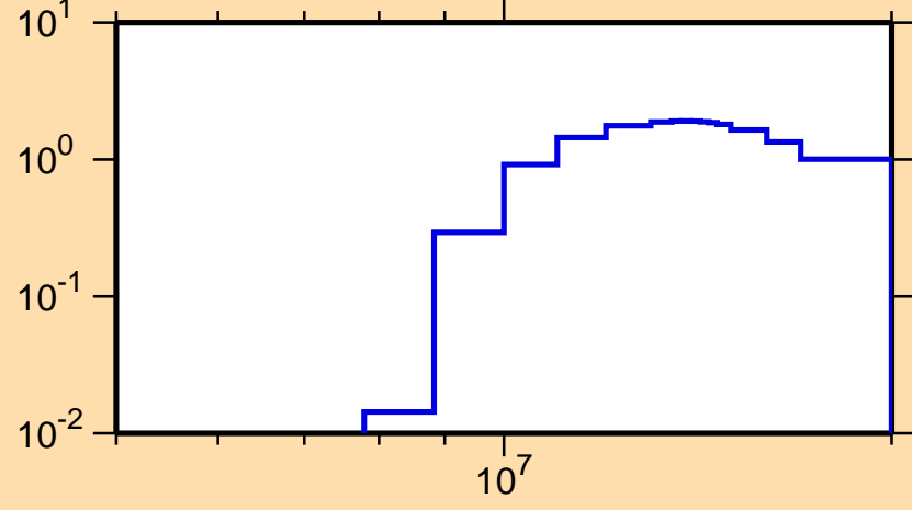
\sigma vs. E for ^{211}\text{Hg}(n,3n)
