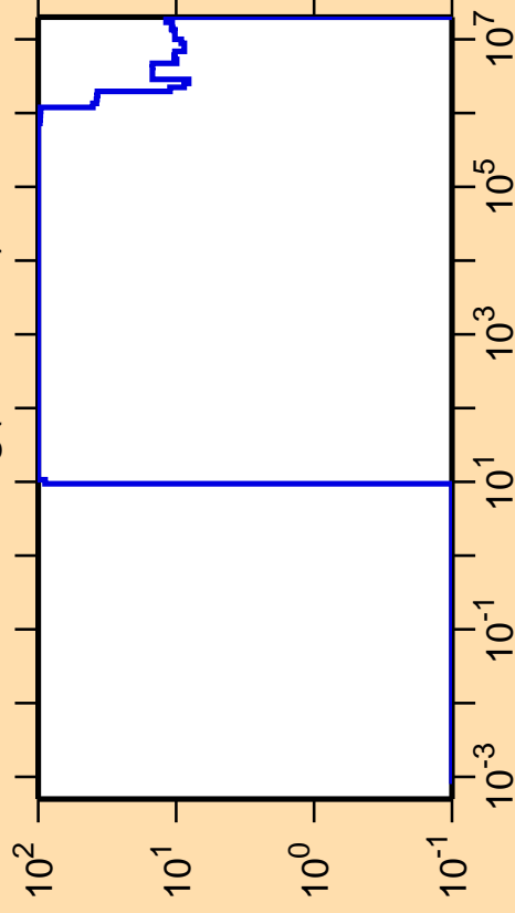
\Delta\sigma/\sigma vs. E for ^{211}\text{Hg}(n,\text{nonel.})
