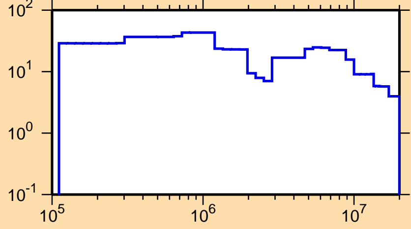
\Delta\sigma/\sigma vs. E for ^{211}\text{Hg}(n,\text{el.})
