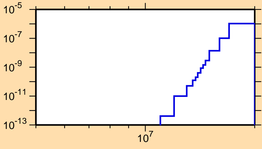
\sigma vs. E for ^{211}\text{Hg}(n,2n\alpha)
