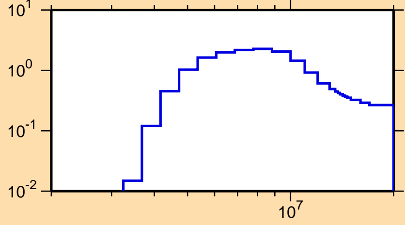
\sigma vs. E for ^{211}\text{Hg}(n,2n)
