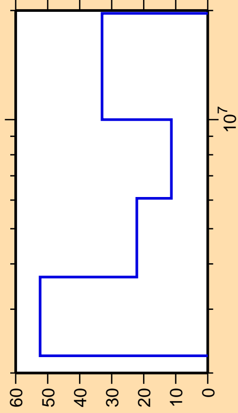
\Delta\sigma/\sigma vs. E for ^{211}\text{Hg}(n,2n)
