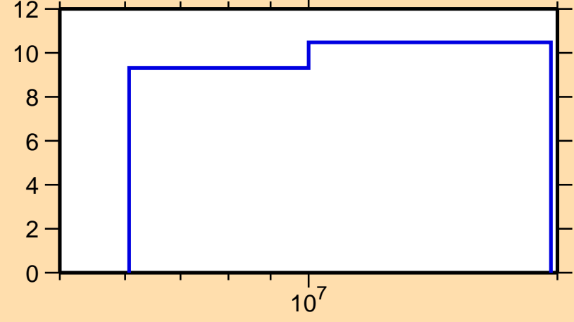
\Delta\sigma/\sigma vs. E for ^{211}\text{Hg}(n,\text{nonel.})
