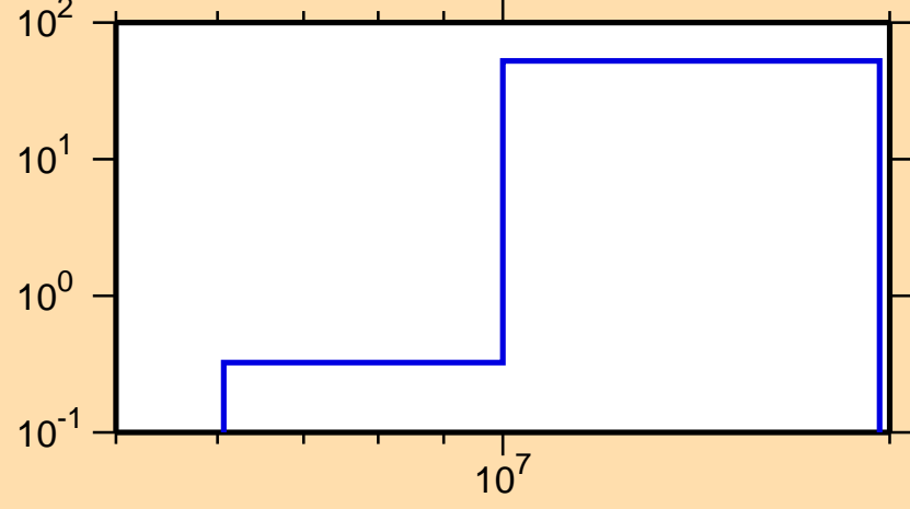
\Delta\sigma/\sigma vs. E for ^{211}\text{Hg}(n,p)
