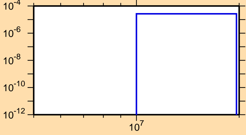
\sigma vs. E for ^{211}\text{Hg}(n,p)
