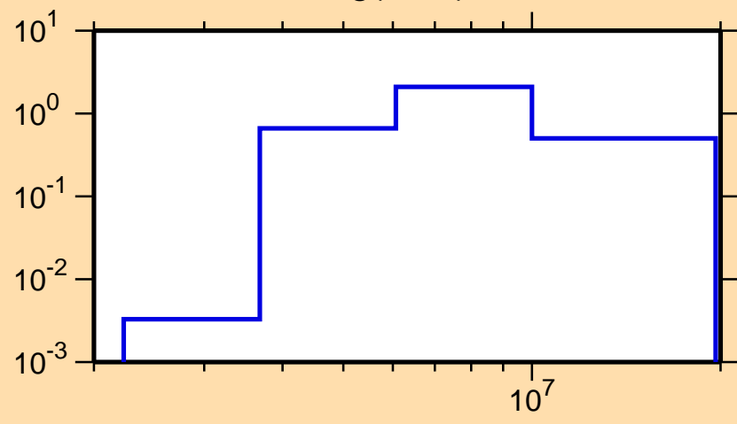
\sigma vs. E for ^{211}\text{Hg}(n,2n)
