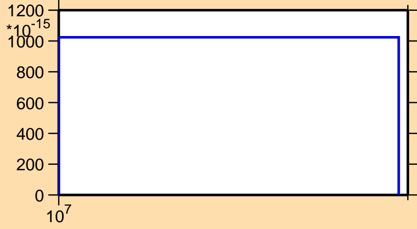
\sigma vs. E for ^{211}\text{Hg}(n,3n\alpha)
