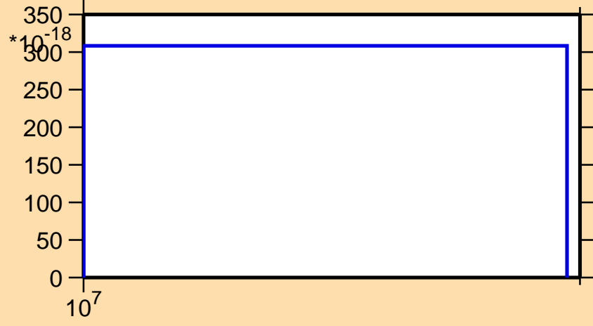
\sigma vs. E for ^{211}\text{Hg} (mt 11)
