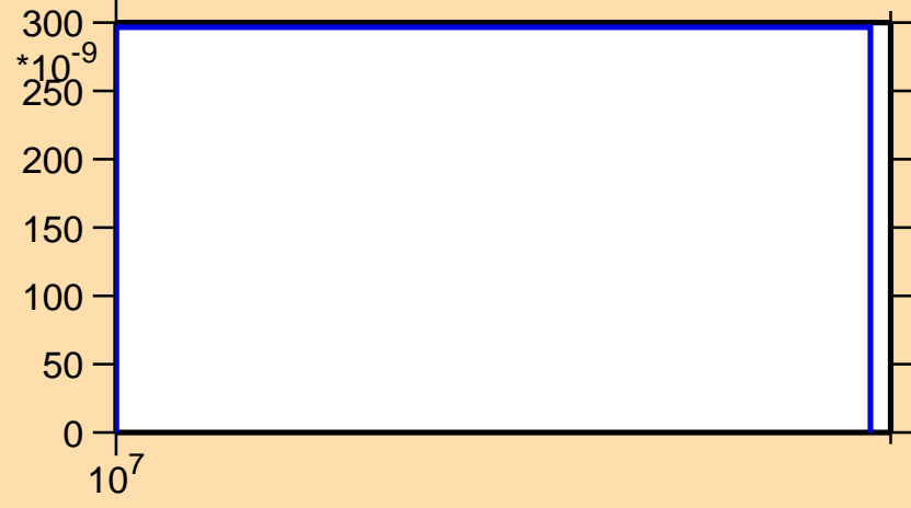
\sigma vs. E for ^{211}\text{Hg}(n,np)
