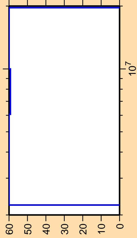
\Delta\sigma/\sigma vs. E for ^{211}\text{Hg}(n,\gamma)
