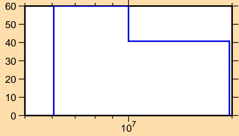
\Delta\sigma/\sigma vs. E for ^{211}\text{Hg}(n,n\text{cont.})
