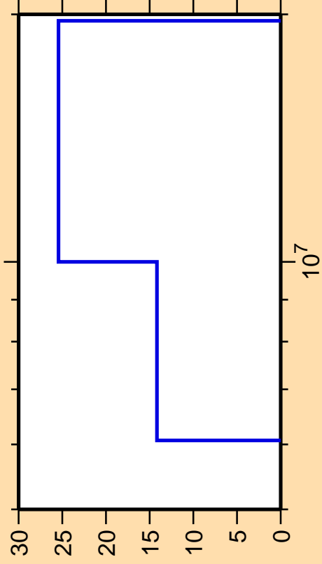
\Delta\sigma/\sigma vs. E for ^{211}\text{Hg}(n,3n)
