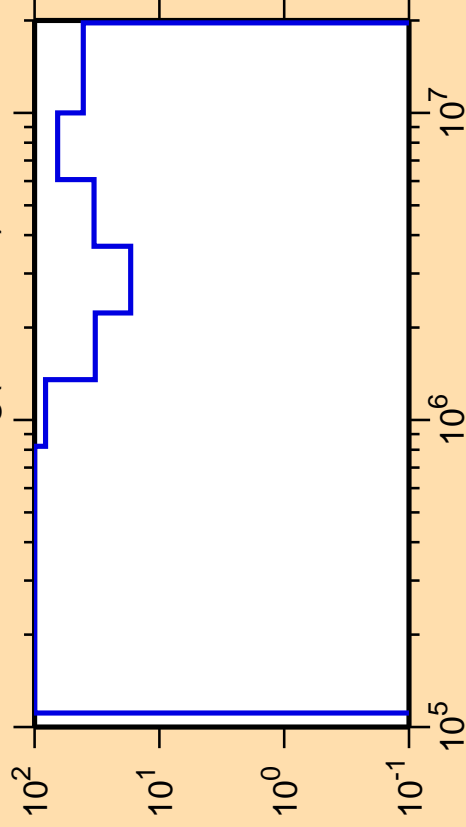
\Delta\sigma/\sigma vs. E for ^{211}\text{Hg}(n,\text{ncont.})
