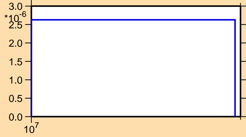
\sigma vs. E for ^{211}\text{Hg}(n,d)
