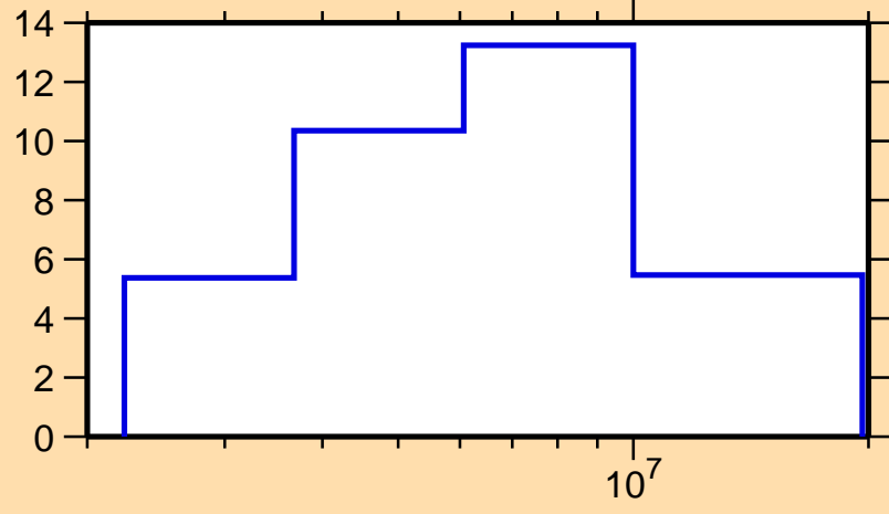
\Delta\sigma/\sigma vs. E for ^{211}\text{Hg}(n,\text{tot.})
