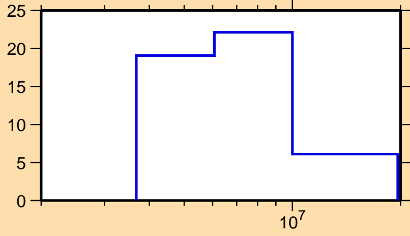
\Delta\sigma/\sigma vs. E for ^{211}\text{Hg}(n,\text{el.})
