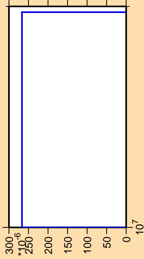
\Delta\sigma/\sigma vs. E for ^{211}\text{Hg} (mt 11)
