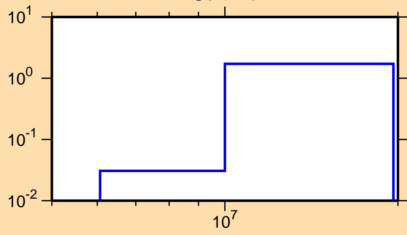
\sigma vs. E for ^{211}\text{Hg}(n,3n)
