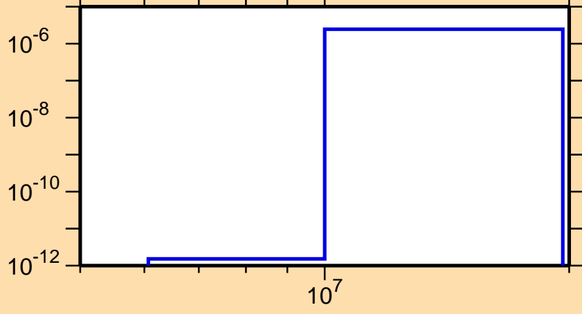
\sigma vs. E for ^{211}\text{Hg}(n,n\alpha)
