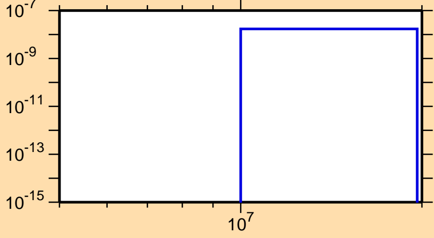
\sigma vs. E for ^{211}\text{Hg}(n,2n\alpha)
