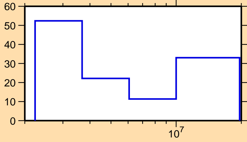
\Delta\sigma/\sigma vs. E for ^{211}\text{Hg}(n,2n)
