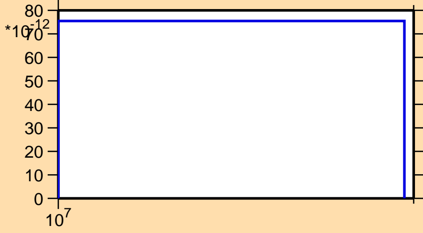
\sigma vs. E for ^{211}\text{Hg}(n,2np)
