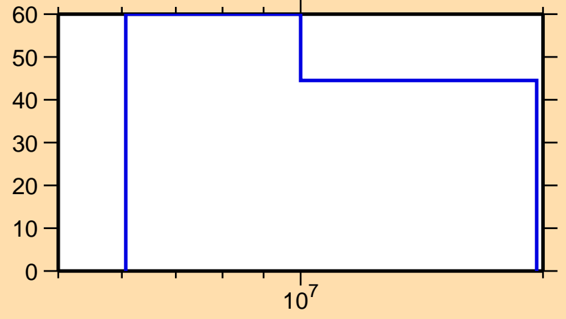
\Delta\sigma/\sigma vs. E for ^{211}\text{Hg}(n,n_1)
