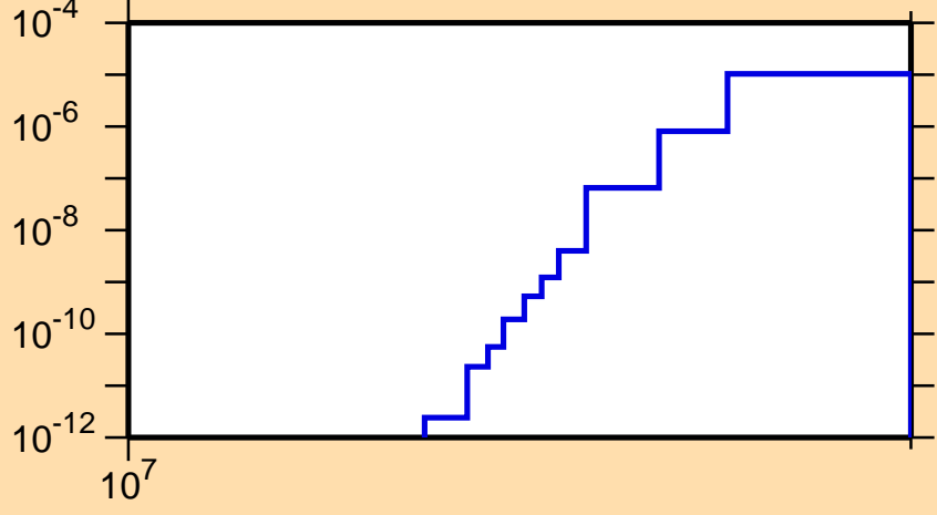
\sigma vs. E for ^{212}\text{Hg}(n,d)
