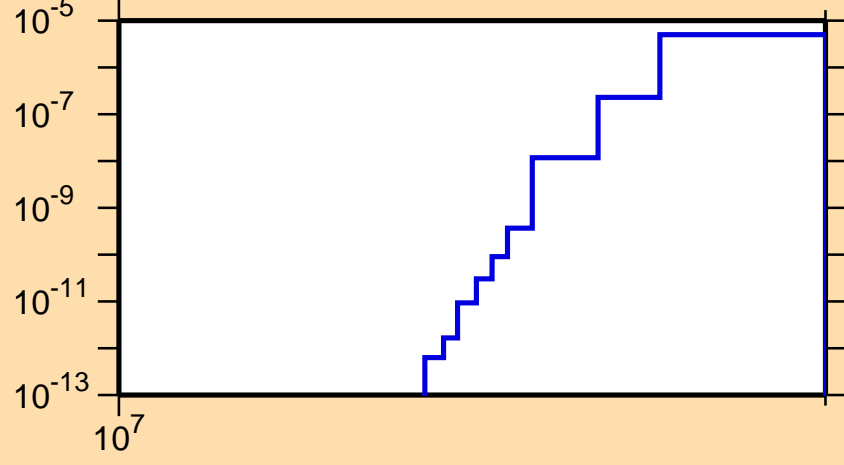
\sigma vs. E for ^{212}\text{Hg}(n,nt)
