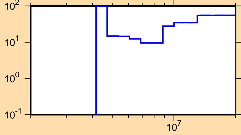
\Delta\sigma/\sigma vs. E for ^{212}\text{Hg}(n,2n)
