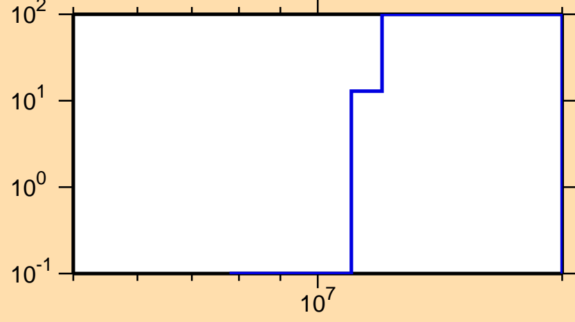
\Delta\sigma/\sigma vs. E for ^{212}\text{Hg}(n,p)
