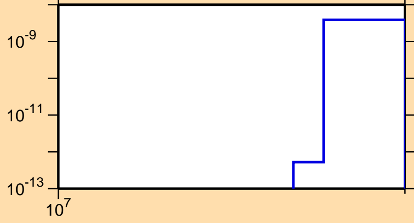
\sigma vs. E for ^{212}\text{Hg}(n,\text{nd})
