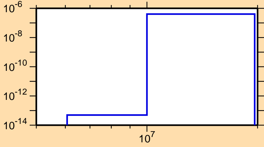
\sigma vs. E for ^{212}\text{Hg}(n,n\alpha)
