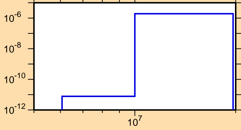
\sigma vs. E for ^{212}\text{Hg}(n,\alpha)
