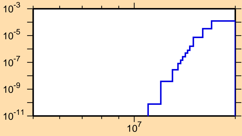
\sigma vs. E for ^{213}\text{Hg}(n,t)
