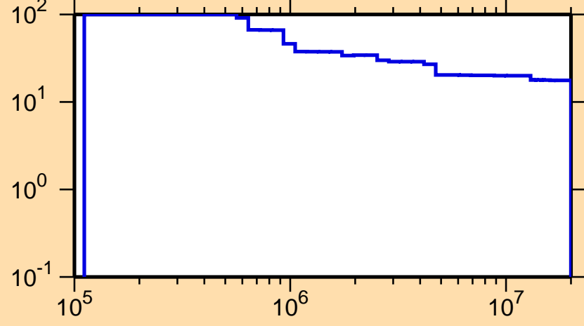
\Delta\sigma/\sigma vs. E for ^{213}\text{Hg}(n,\text{nonel.})
