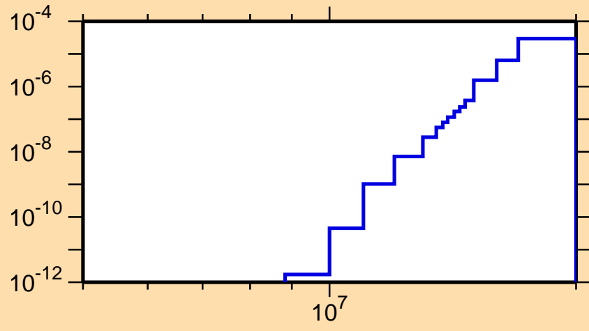
\sigma vs. E for ^{213}\text{Hg}(n,\alpha)
