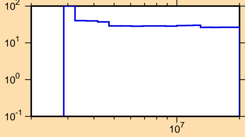
\Delta\sigma/\sigma vs. E for ^{213}\text{Hg}(n,2n)
