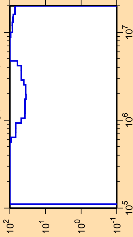
\Delta\sigma/\sigma vs. E for ^{213}\text{Hg}(n,\text{ncont.})
