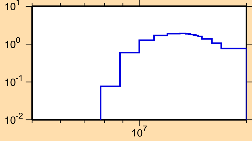
\sigma vs. E for ^{213}\text{Hg}(n,3n)
