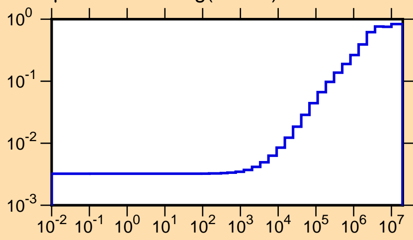
\mu vs. E for ^{213}\text{Hg}(\text{mt251})
