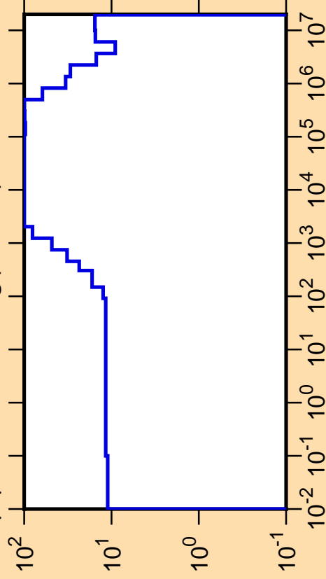
\Delta\mu/\mu vs. E for ^{213}\text{Hg}(\text{mt251})
