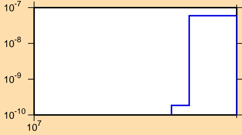
\sigma vs. E for ^{215}\text{Hg}(n,\text{nd})
