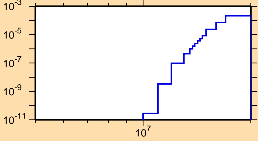
\sigma vs. E for ^{215}\text{Hg}(n,p)
