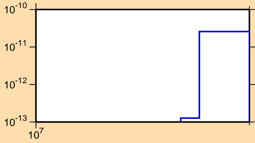
\sigma vs. E for ^{215}\text{Hg}(n,3n\alpha)
