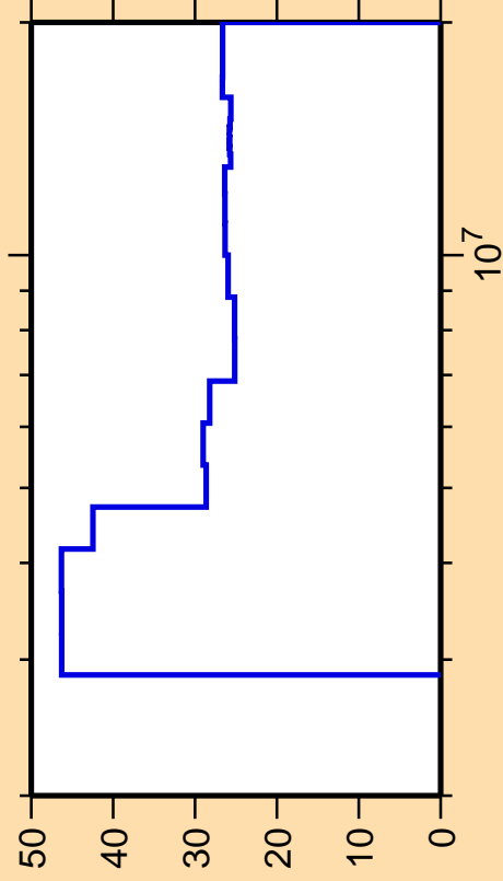
\Delta\sigma/\sigma vs. E for ^{215}\text{Hg}(n,n\text{cont.})
