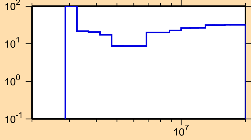
\Delta\sigma/\sigma vs. E for ^{215}\text{Hg}(n,2n)
