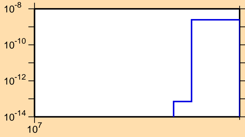
\sigma vs. E for ^{215}\text{Hg}(n,2np)
