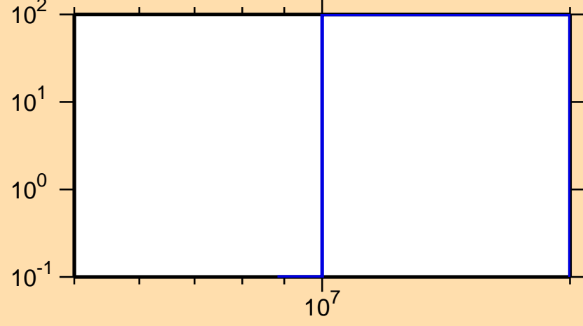
\Delta\sigma/\sigma vs. E for ^{215}\text{Hg}(n,p)
