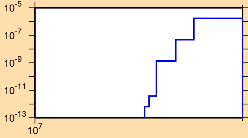
\sigma vs. E for ^{215}\text{Hg}(n,np)
