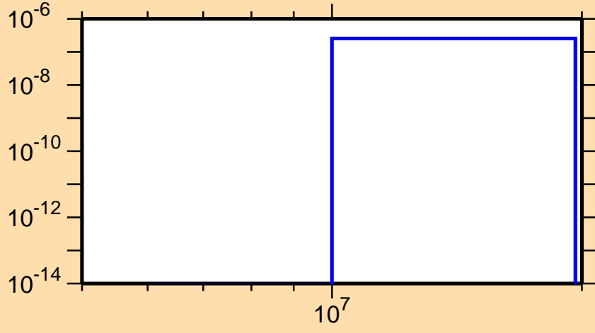
\sigma vs. E for ^{215}\text{Hg}(n,n\alpha)
