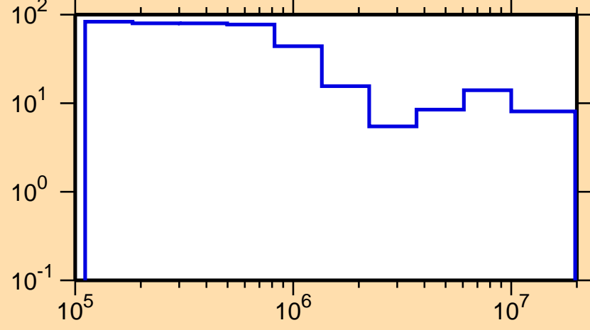
\Delta\sigma/\sigma vs. E for ^{215}\text{Hg}(n,\text{tot.})
