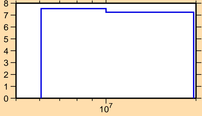
\Delta\sigma/\sigma vs. E for ^{215}\text{Hg}(n,\text{nonel.})
