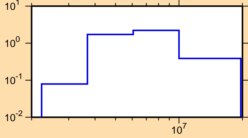
\sigma vs. E for ^{215}\text{Hg}(n,2n)
