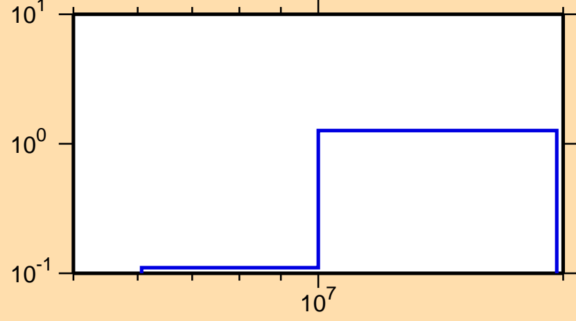
\sigma vs. E for ^{215}\text{Hg}(n,3n)
