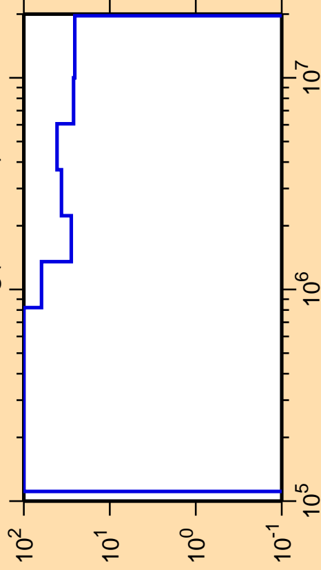
\Delta\sigma/\sigma vs. E for ^{215}\text{Hg}(n,\text{ncont.})
