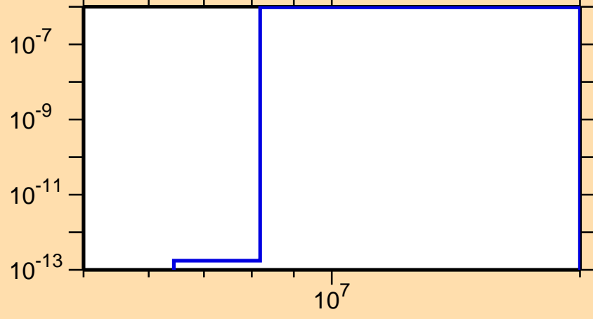
\sigma vs. E for ^{215}\text{Hg}(n,\alpha)
