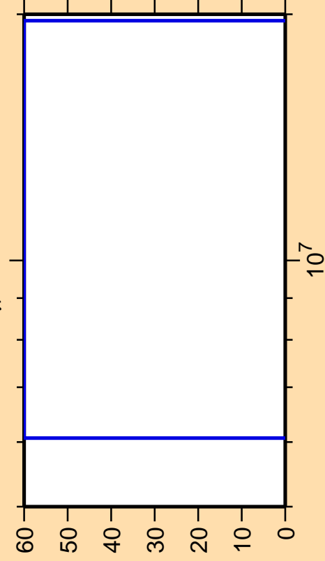
\Delta\sigma/\sigma vs. E for ^{268}\gamma
