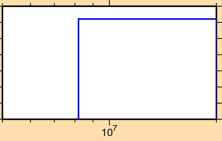
\sigma vs. E for ^{268}\text{He3} )
