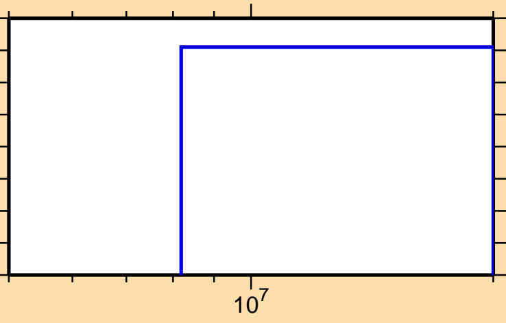
\sigma vs. E for ^{268}
