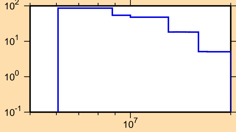
\Delta\sigma/\sigma vs. E for ^{269}
