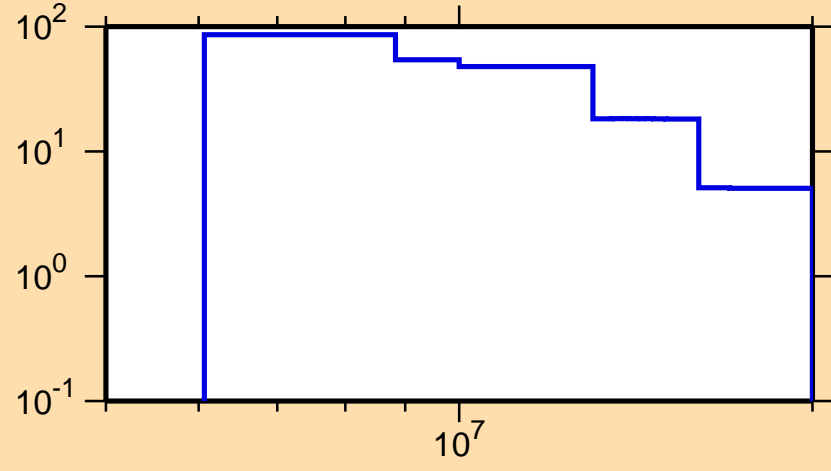
\Delta\sigma/\sigma vs. E for ^{269}\text{Ac}
