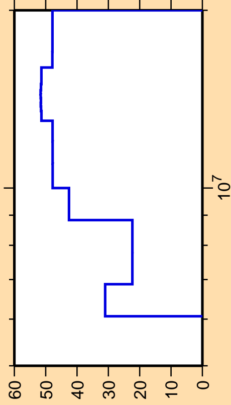
\Delta\sigma/\sigma vs. E for ^{269}\text{Ac}
