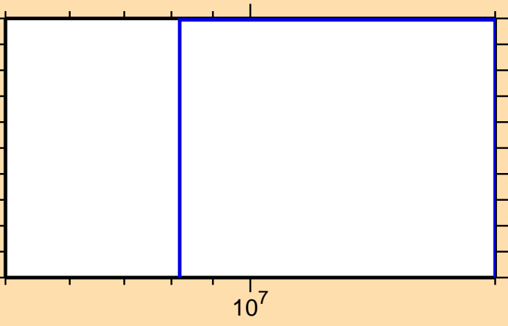
\sigma vs. E for ^{269}
