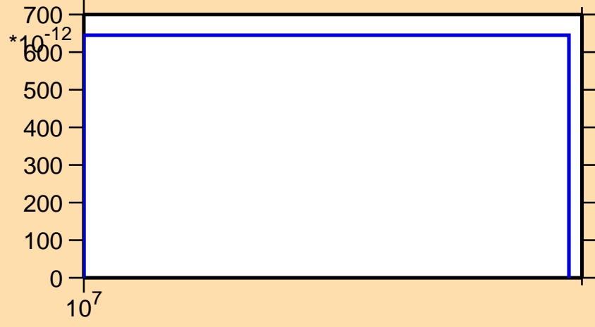
\sigma vs. E for ^{111}\text{I} (mt 34)
