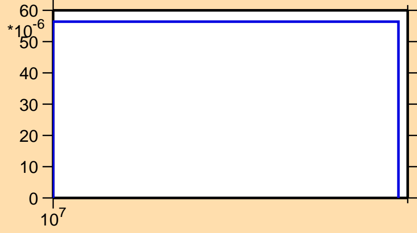
\sigma vs. E for ^{111}\text{I}(n,2n)
