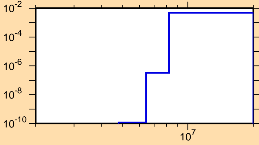
\sigma vs. E for ^{111}\text{I}(n,\text{pd})
