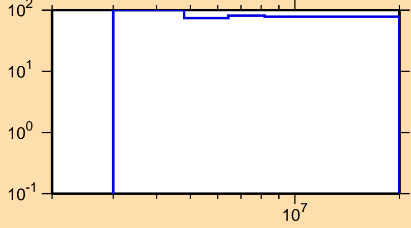
\Delta\sigma/\sigma vs. E for ^{111}\text{I}(n,ncont.)
