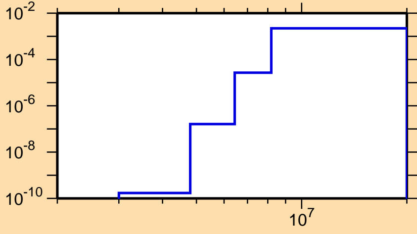
\sigma vs. E for ^{111}\text{I} (mt 45)
