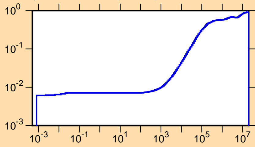
\mu vs. E for ^{112}\text{I}(\text{mt251})
