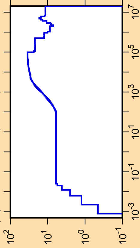
\Delta\mu/\mu vs. E for ^{112}\text{I}(\text{mt251})
