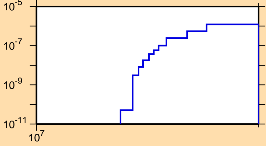
\sigma vs. E for ^{112}\text{I}(n,2n\alpha)
