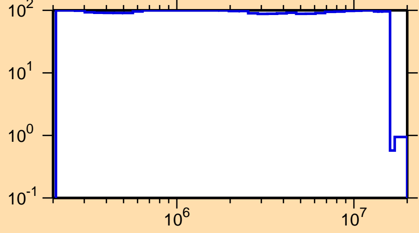
\Delta\sigma/\sigma vs. E for ^{112}\text{I}(n,n_1)
