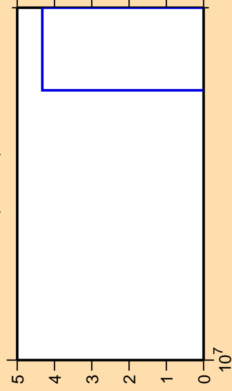
\Delta\sigma/\sigma vs. E for ^{112}\text{I}(n,3n\alpha)
