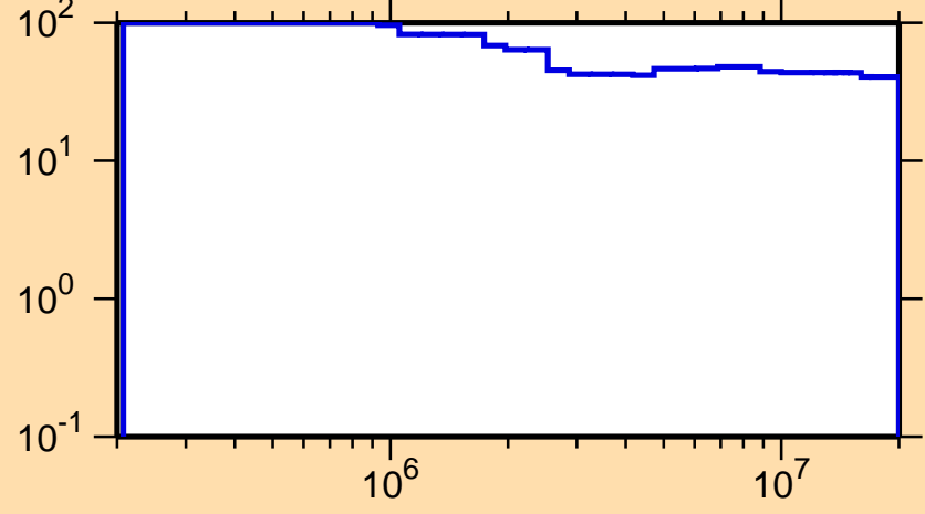
\Delta\sigma/\sigma vs. E for ^{112}\text{I}(n,\text{inel.})
