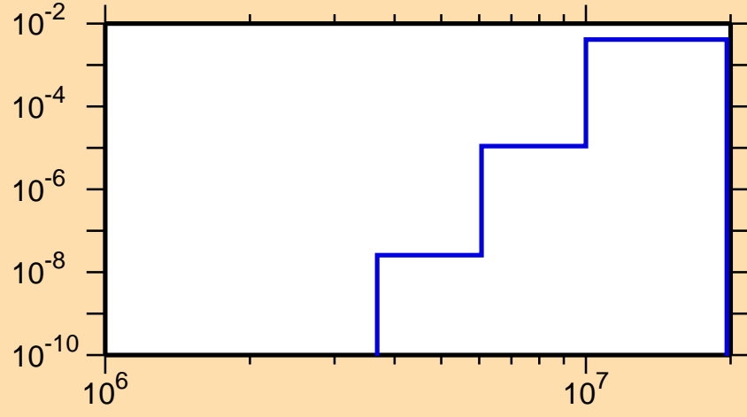
\sigma vs. E for ^{112}\text{I}(n,\text{He3})
