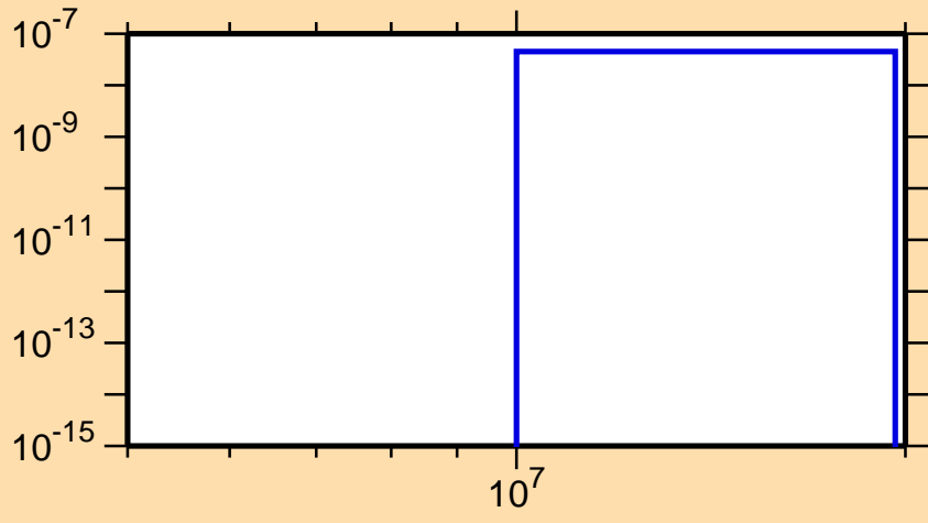
\sigma vs. E for ^{112}\text{I}(\text{mt 34})
