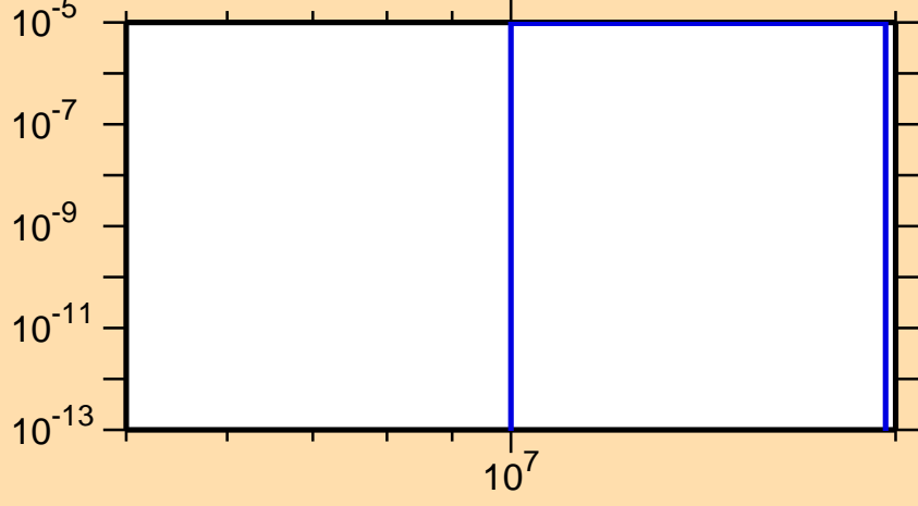
\sigma vs. E for ^{112}\text{I}(n,nd)
