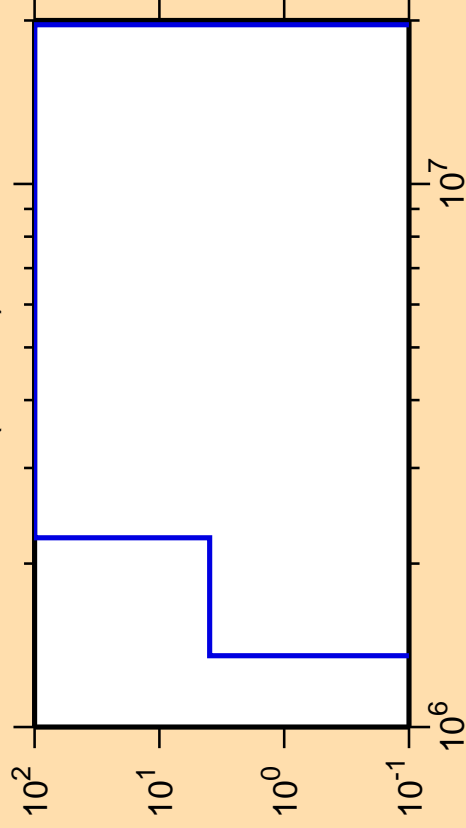
\Delta\sigma/\sigma vs. E for ^{112}\text{I}(n,\text{He3})
