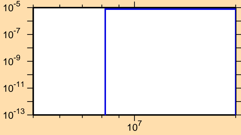
\sigma vs. E for ^{112}\text{I}(n,\text{nd})
