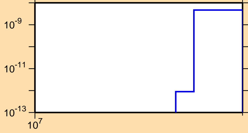
\sigma vs. E for ^{113}\text{I}(n,nt)
