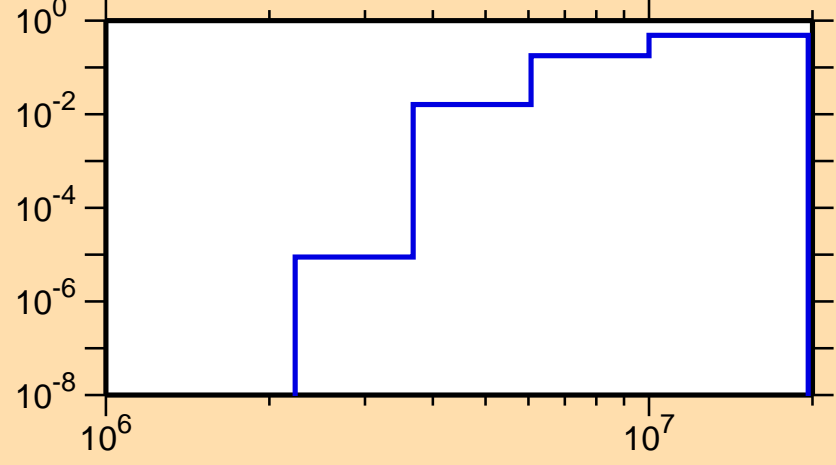
\sigma vs. E for ^{113}\text{I}(n,np)
