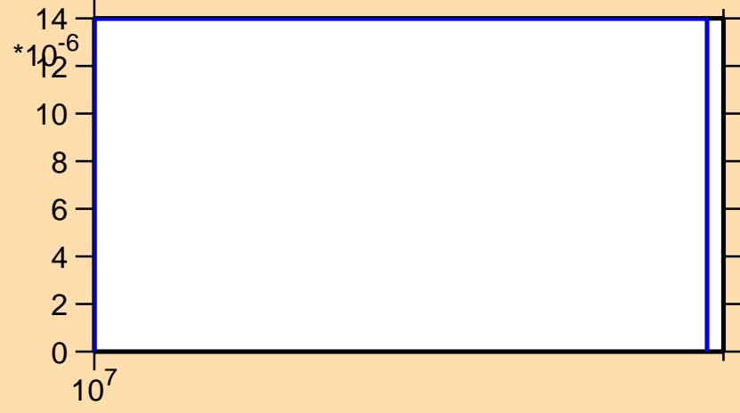
\sigma vs. E for ^{113}\text{I}(n,2np)
