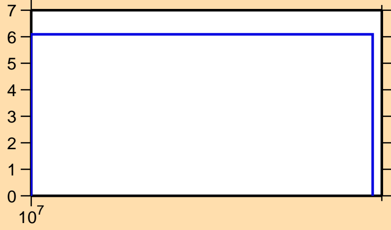
\Delta\sigma/\sigma vs. E for ^{113}\text{I}(n,\text{nonel.})
