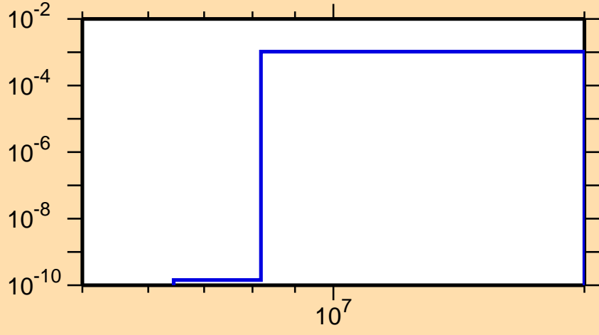
\sigma vs. E for ^{113}\text{I}(n,\text{pd})
