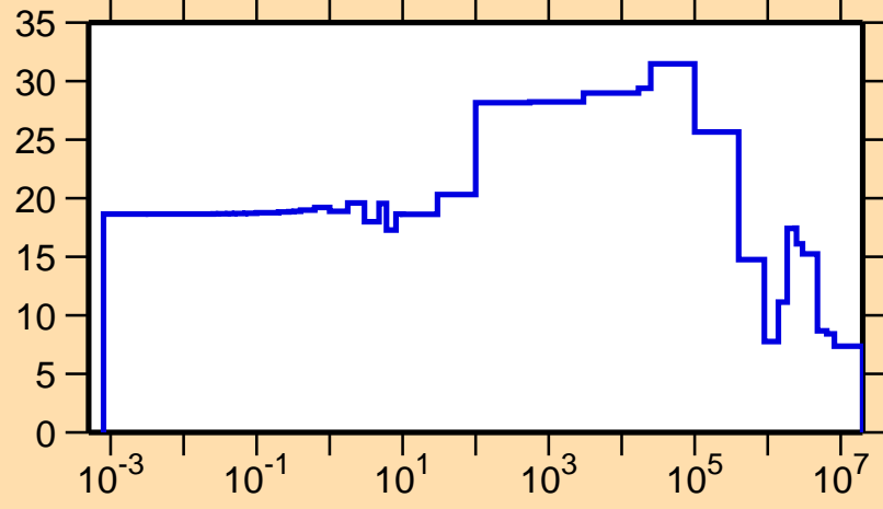
\Delta\sigma/\sigma vs. E for ^{113}\text{I}(n,el.)
