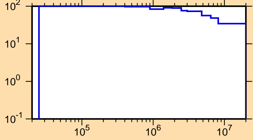
\Delta\sigma/\sigma vs. E for ^{113}\text{I}(n,n_1)
