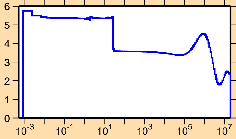
\sigma vs. E for ^{114}\text{I}(n,\text{el.})
