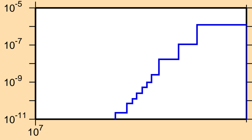
\sigma vs. E for ^{114}\text{I} (mt 34)
