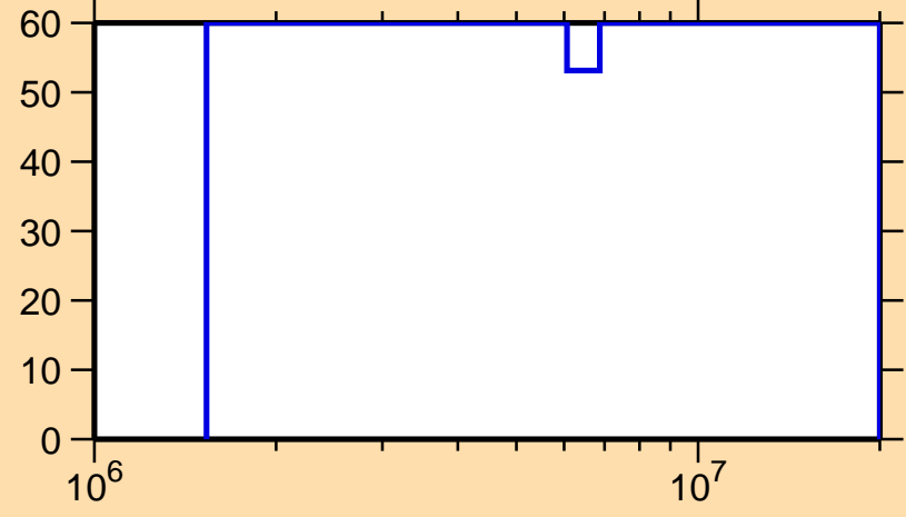
\Delta\sigma/\sigma vs. E for ^{114}\text{I}(n,ncont.)
