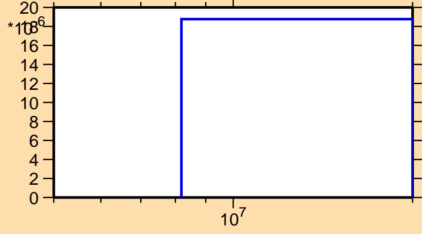
\sigma vs. E for ^{114}\text{I}(n,\text{pt})
