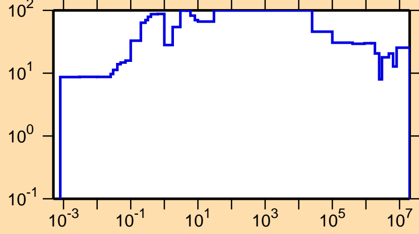
\Delta\sigma/\sigma vs. E for ^{114}\text{I}(n,\text{tot.})
