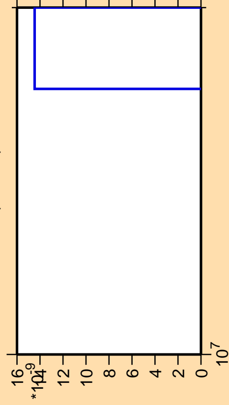
\Delta\sigma/\sigma vs. E for ^{115}\text{I}(n,3n\alpha)
