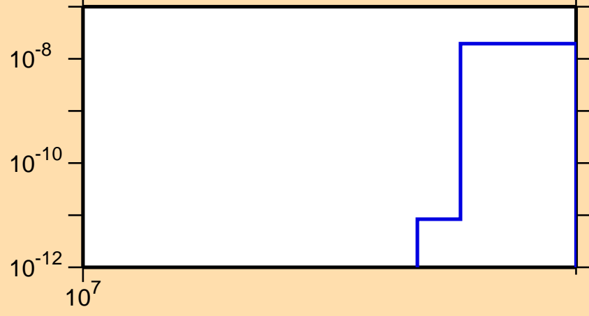
\sigma vs. E for ^{115}\text{I}(n,nt)
