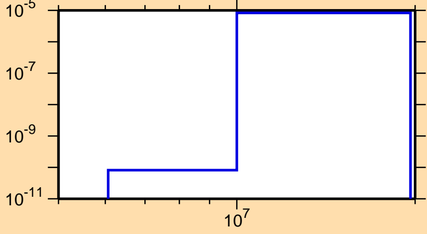
\sigma vs. E for ^{115}\text{I}(\text{mt117})
